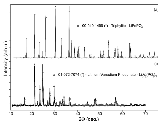
Fig. 2. X-ray diffraction patterns of the \text{LiFePO}_4/\text{carbon} (a) and \text{Li}_3\text{V}_2(\text{PO}_4)_3/\text{carbon} (b) composite samples
