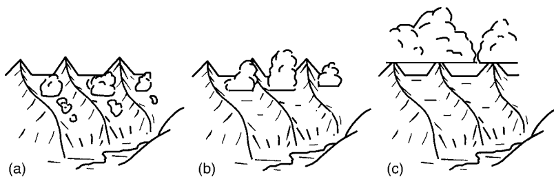
Fig. 4.11 Observation of the daytime growth of cumulus over south-facing slopes in alpine terrain: (a) 0700 UTC; (b) 0900 UTC; (c) 1300 UTC (from Tucker, 1954).
