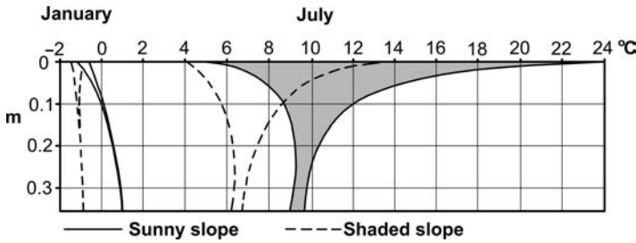
Fig. 2.43 Daily mean maximum and minimum soil temperatures to 35 cm depth on sunny and shaded slopes near the tree line, Davos (2170 m) in January and July 1968–70 (after Turner et al. , 1975).
