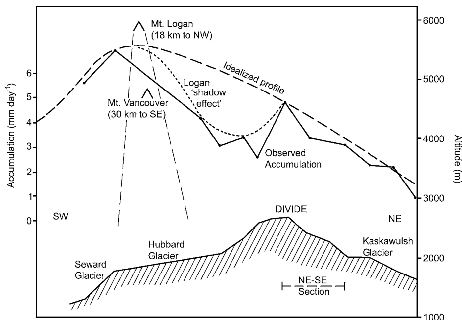
Fig. 5.23 Observed and idealized profiles of accumulation rate ( \text{mm day}^{-1} ) across the St. Elias Range based on snow-pit data (after Taylor-Barge, 1969).
