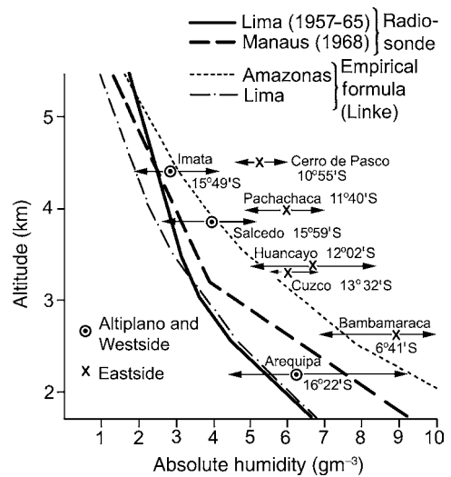
Fig. 2.5 Annual averages and range of monthly means of absolute humidity ( \text{g m}^{-3} ) as a function of altitude in tropical South America (after Prohaska, 1970). Station data, free air radiosonde values, and gradients calculated from Linke's equation are shown.
