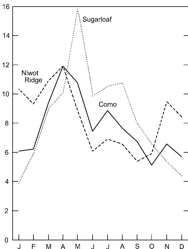
Fig. 5.19 Precipitation regimes on the east slope of the Front Range, Colorado ( 40^{\circ} N, 105.5^{\circ} W) expressed as monthly percentages of the annual total (based on Niwot Ridge LTER data). Niwot Ridge (3743 m) is 2.5 km east of the Continental Divide, Como (3022 m) is 9.5 km east of the Divide and Sugarloaf (2591 m) 22.5 km east of the Divide. The data for Niwot Ridge and Como are for 1952–2004, for Sugarloaf for 1952–1991.
