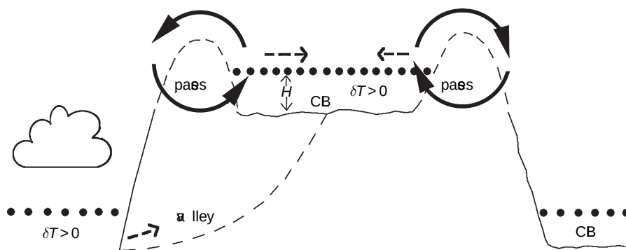
Fig. 3.50 Schematic diagram of the diurnal circulation over the Bolivian Altiplano (from Egger et al. , 2005; Fig. 1).
