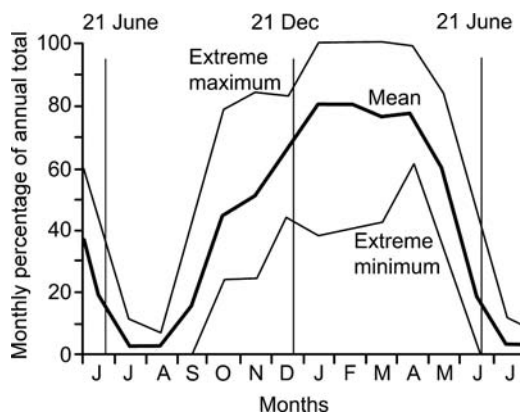
Fig. 5.18 Percentage of the monthly precipitation falling as snow on Ben Nevis (1343 m), 1895–1904. Average (solid) and extremes (fine lines) (after Thom, 1974).
