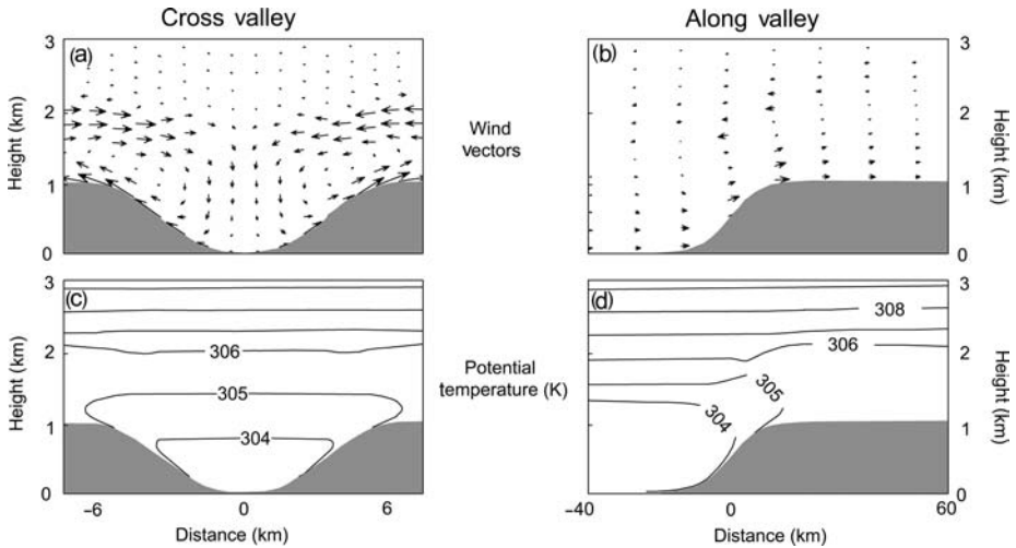
Fig. 3.37 Sections of wind vectors and potential temperature, respectively, (a) and (c) cross-valley and (b) and (d) along-valley, for a WRF model simulation with three-dimensional plains–valley topography. The cross-sections are 20 km upvalley (from Rampanelli et al. , 2004).
