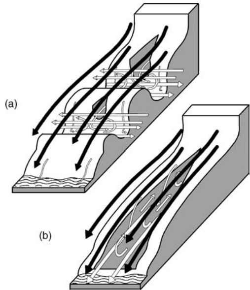
Fig. 3.46 A model of nocturnal airflow over the Drakensberg foothills in winter (from Tyson and Preston-Whyte, 1972). (a) Valleys normal to mountains and coastline (b) valleys parallel to the slope.
