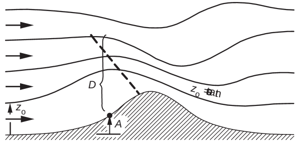
Fig. 2.27 Schematic illustration of streamlines over a hill showing phase tilt upwind (dashed line) (from Smith, 1990).
