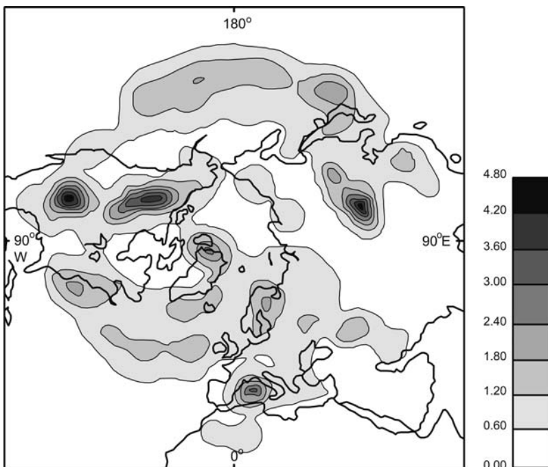
Fig. 3.11 The density of cyclogenesis (per 10^6 \text{ km}^2 per month) in the northern hemisphere analyzed from ECMWF ERA-15 reanalysis data, updated with operational analyses, for December–February, 1979–2000 (from Hoskins and Hodges, 2002).
