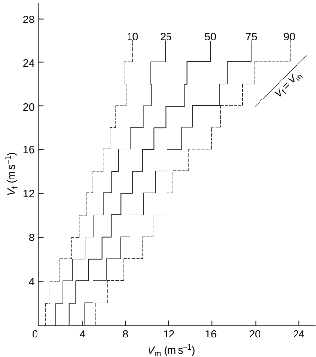
Fig. 2.26 Wind speeds observed on mountain summits ( V_m ) in Europe and at the same level in the free air ( V_f ) (from Wahl, 1966).
