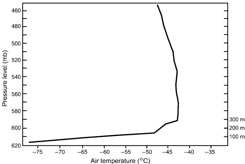
Fig. 5.25 The temperature in the lower troposphere in the austral summer, 2 July 1966, at Plateau Station (79° 15' S, 40° 30' E, 3625 m), East Antarctica (after Kuhn, 2004).
