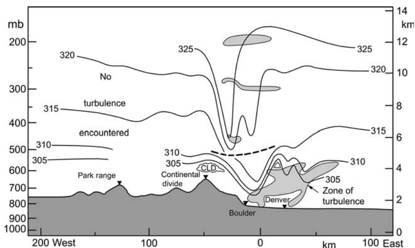
Fig. 3.31 A cross-section of potential temperature K based on aircraft data during a windstorm in Boulder on 11 January 1972. The dashed line separates data collected at different times. The three bands of turbulence above Boulder were recorded along horizontal flight paths and are probably continuous vertically (after Lilly, 1978).
