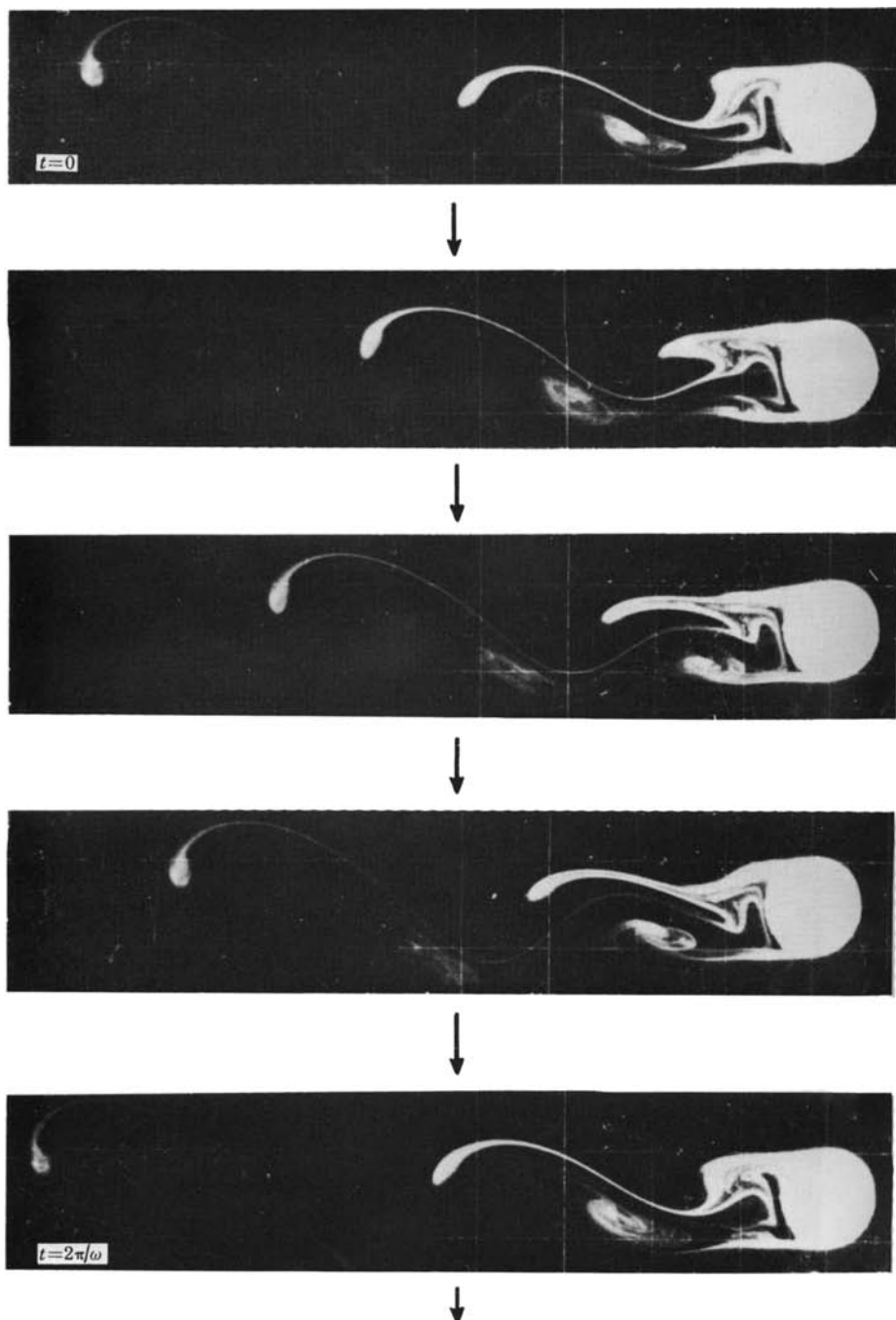
Fig. 3.26 Laboratory model of vortex shedding (D. J. Boyer and the Royal Society, London Phil. Trans. 1982, plate 6, pp. 542). Laboratory model of double eddy formation in the lee of a cylindrical obstacle for easterly flow in a rotating water tank. Motion in the larger eddy at the right-hand edge of the obstacle, viewed downstream, circulates cyclonically, while motion in the smaller detached eddy at the left side is anticyclonic.
