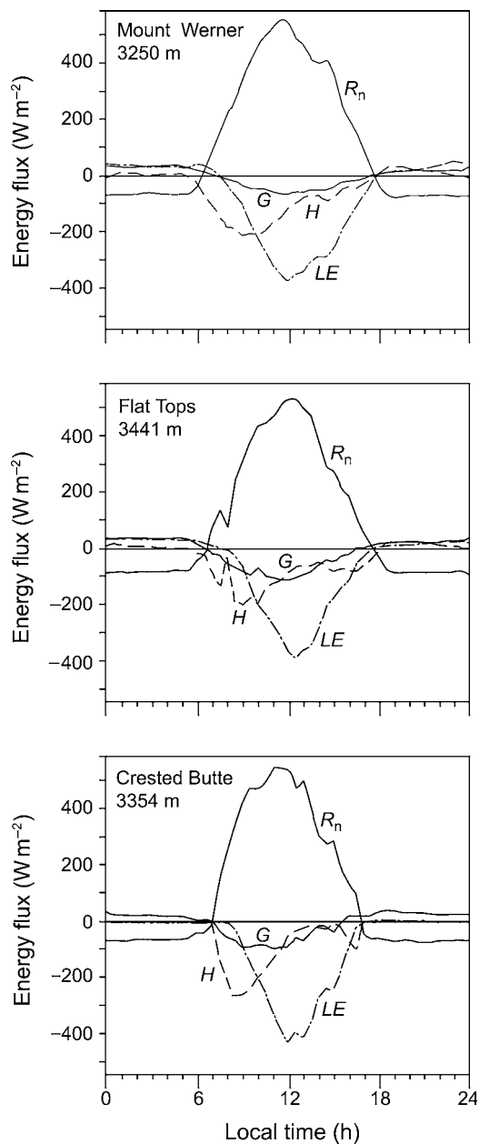
Fig. 4.1 The diurnal variation of surface energy fluxes averaged for 23–31 August 1985 at Mt. Werner (40.5° N, 106.7° W, 3250 m), Flat Tops (40.0° N, 107.3° W, 3441 m) and Crested Butte (38.9° N, 107.9° W, 3354 m), Colorado (adapted from Bossert and Cotton, 1994).
