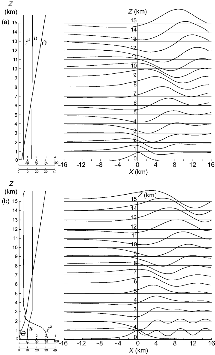
Fig. 3.18 Calculated streamlines showing wave development over a ridge for two idealized profiles of wind speed ( u ) and potential temperature ( \theta ) (from Sawyer, 1960). Values of l^2 are also shown (see text). In (a) u and l^2 are constant with height; in (b) l^2 is large in the lowest layer and then decreases rapidly to low values.
