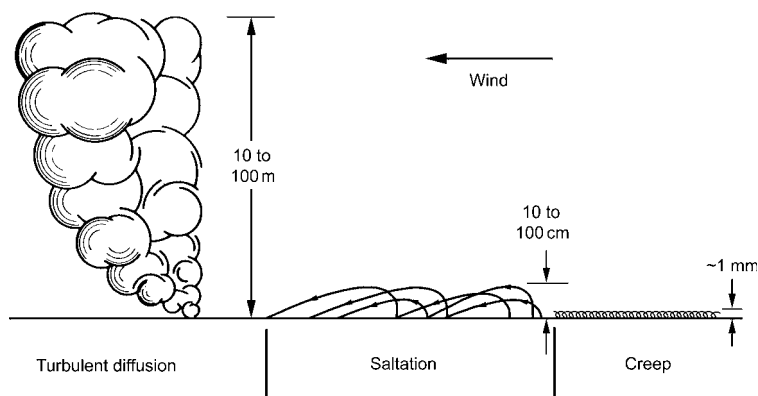
Fig. 4.35 Modes of snow transport by the wind (from Mellor, 1965).
