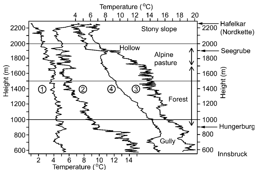
Fig. 4.5 Slope temperatures on the Nordkette, Innsbruck, 2 April 1930 (after Wagner, 1930).
