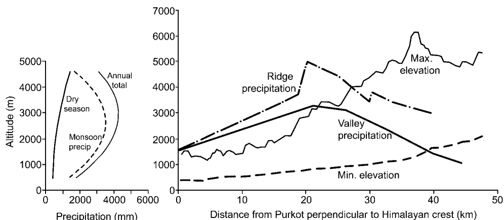
Fig. 5.4 Precipitation gradients in the Annapurna region (adapted from Putkonen, 2004). Left: Altitudinal profile of October–May (solid), June–September (dashed) and annual precipitation. Right: A south–north transect of total precipitation for 1 September 2000–31 August 2001 from Purkhot to the main crest of the Himalaya (after Putkonen, 2004).
