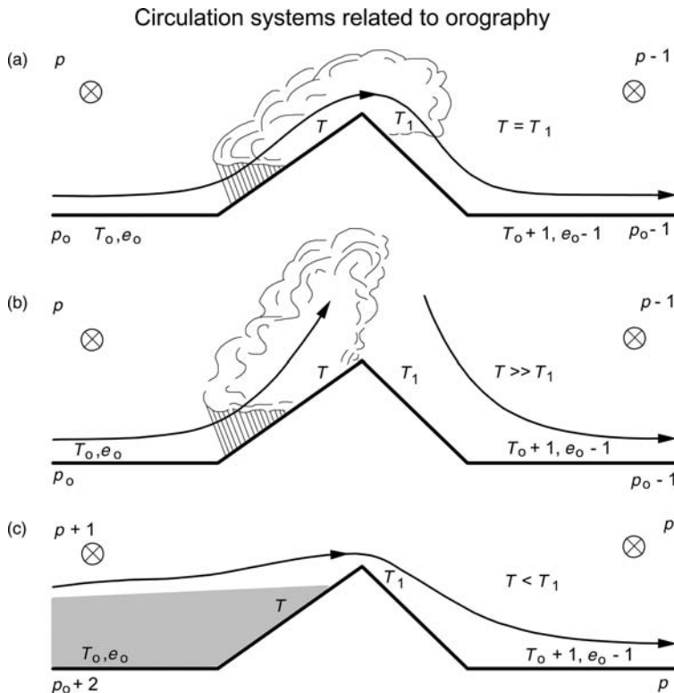
Fig. 3.29 Three types of föhn. (a) Cyclonic föhn in a stable atmosphere with strong winds; (b) cyclonic föhn in a less stable atmosphere; and (c) anticyclonic föhn with a damming up of cold air (after Cadez, 1967; from Yoshino, 1975).
