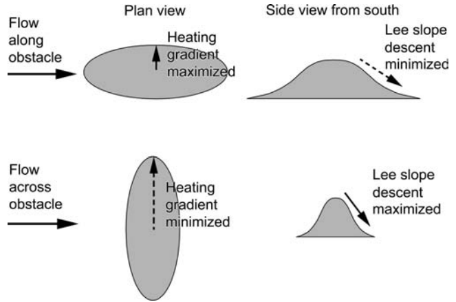
Fig. 2.30 Schematic illustration of the forcing and response of airflow along (above) and across (below) a heated barrier (from Crook and Turner, 2005).
