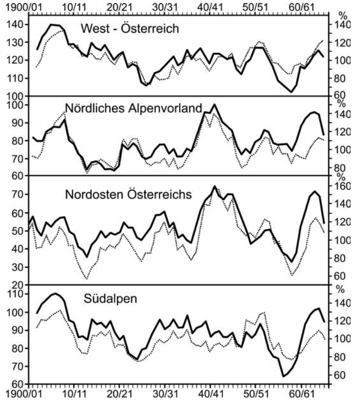
Fig 7.3 Secular trends from 1900–1 to 1965–6 in the number of days with snow cover and total new snowfall as a percentage of the 1900–1 to 1959–60 mean value for four regions in Austria: western Austria, northern Alpine Foreland, northeast Austria, and southern Alps (from Steinhauser, 1970).
