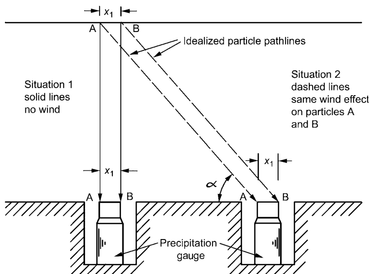
Fig. 4.31 The absence of any direct effect of the inclination angle of falling precipitation on gauge catch (from Peck, 1972a).
