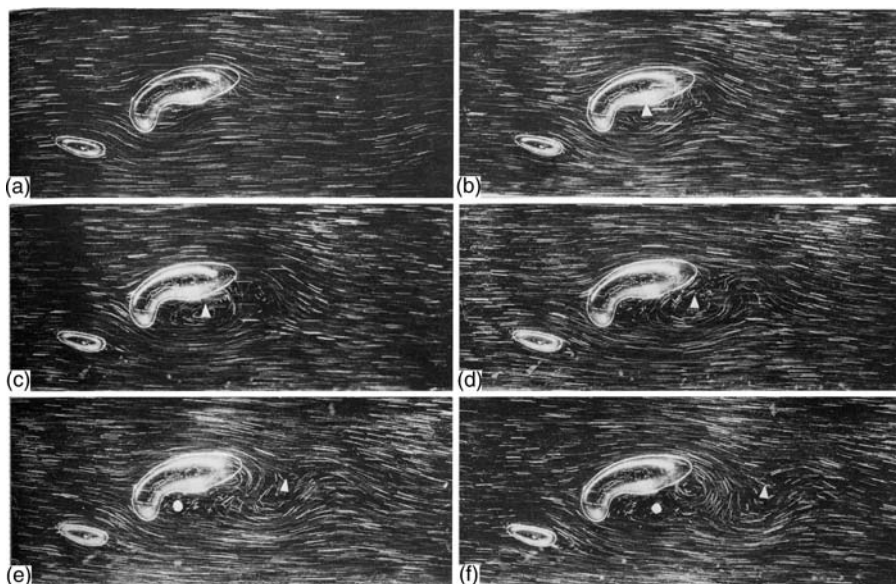
Fig. 3.12 Cyclonic eddies forming in westerly flow over a model Alpine/Pyrenean topography. The laboratory experiment uses a towed obstacle in a linearly stratified rotating water channel 2.4 m long, 0.4 m wide and 0.3 m deep. The flow evolves from (a) 13 h equivalent atmospheric time through (b) 26 h (c) 39 h (d) 52 h (e) 65 h and (f) 78 h, respectively. The triangle marks the center of the first cyclone and the circle the second; flow splitting occurs at the western end of the Alps (D. J. Boyer and Met. Atmos. Physics 1987, Springer).
