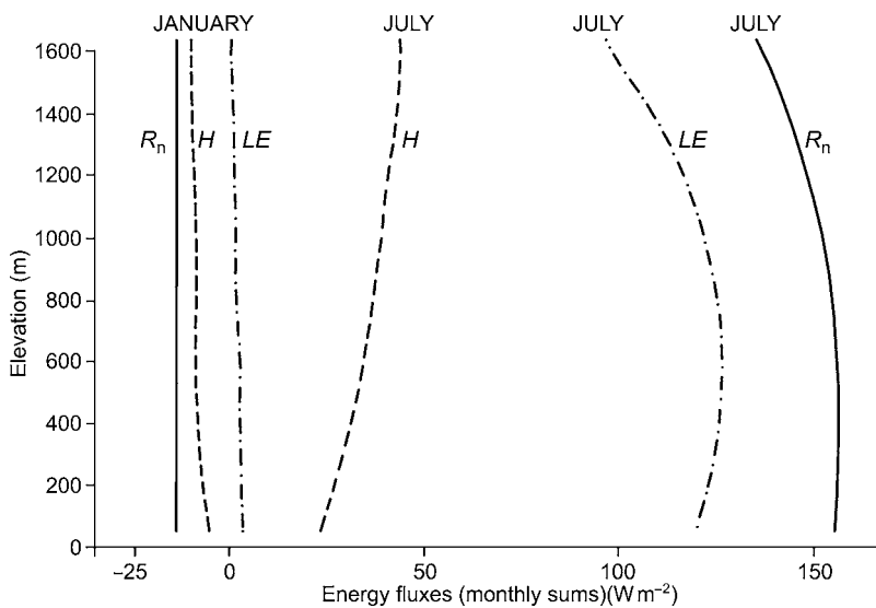
Fig. 4.4 Seasonal variations of net radiation and turbulent heat fluxes with altitude in Croatia (after Pleško and Šinik, 1978).
