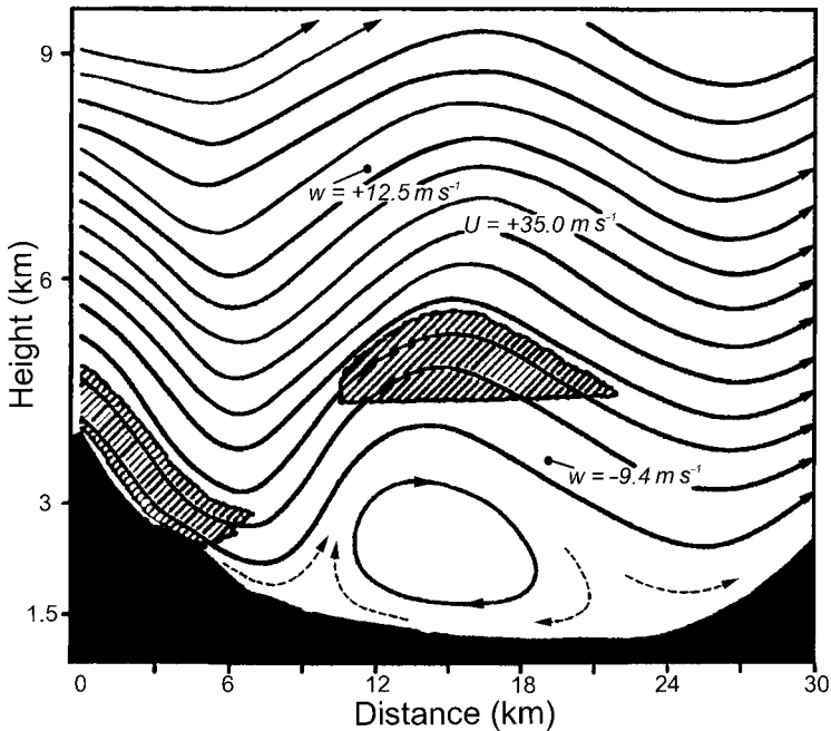
Fig. 3.21 Streamlines for 16 February 1952 in the lee of the Sierra Nevada, based on glider measurements, showing a large rotor and lenticular wave cloud (adapted from Holmboe and Klieforth, 1957).
