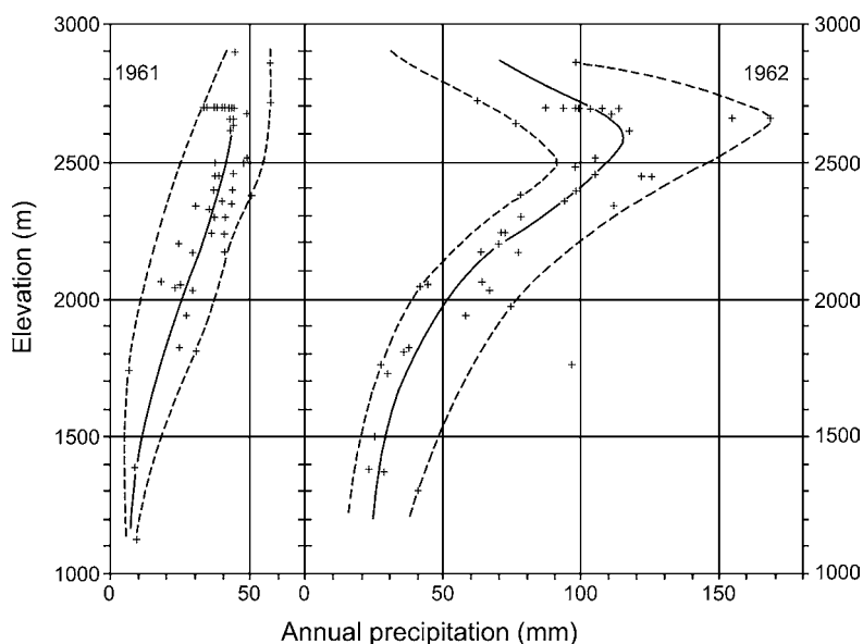
Fig. 5.7 Annual rainfall (mm) versus altitude in the Hoggar in a wet year and dry year (after Yacono, 1968).
