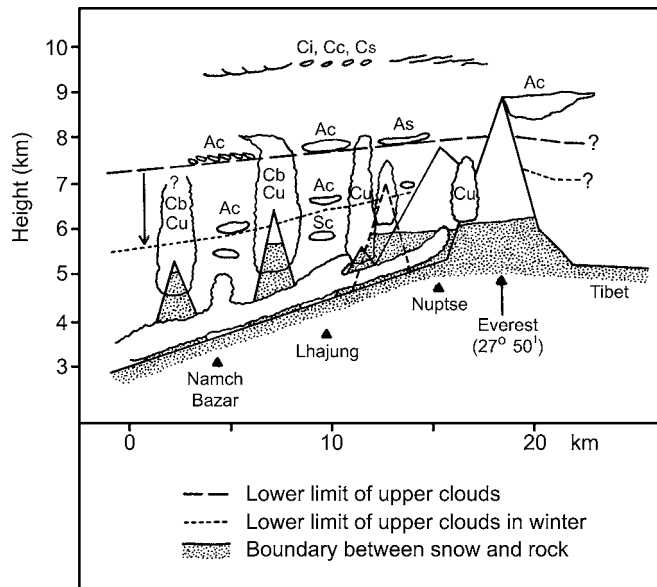
Fig. 5.5 Schematic cloud patterns in summer and winter in the Khumbu region, Nepal (after Yasunari, 1976a). Ac, altocumulus; As, altostratus; Ci, cirrus; Cc, cirrocumulus; Cu, cumulus; Cb, cumulonimbus; Cs, cumulostratus.
