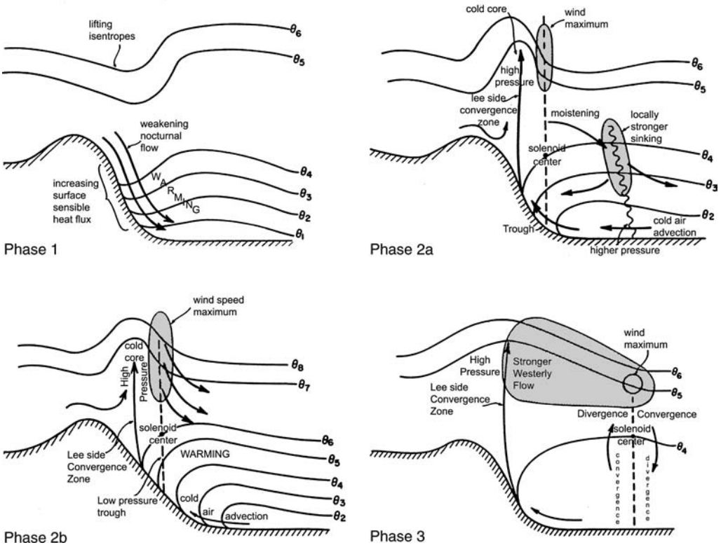
Fig 3.49 Conceptual model of a mountain-plains circulation east of the Front Range, Colorado (from Wolyn and McKee, 1994).
