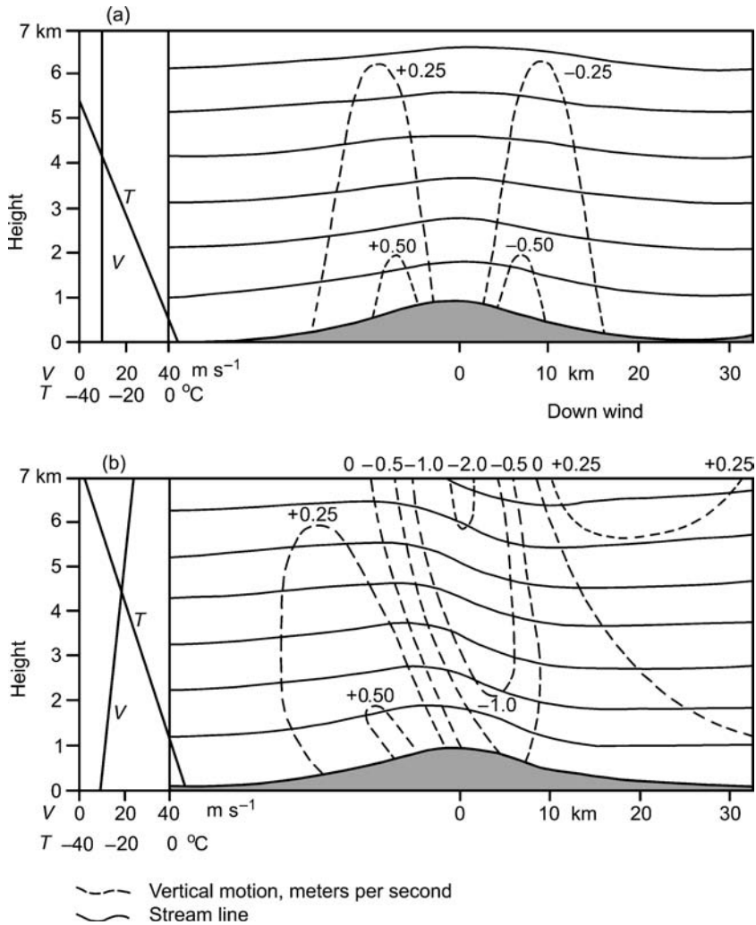
Fig. 4.25 Orographically induced vertical motion for a simple barrier with westerly flow: (a) f(z) = 0 ; (b) k = 0 (from Walker, 1961). The solid lines are streamlines; the dashed lines are vertical motion ( \text{m s}^{-1} ). The assumed gradients of wind speed and temperature are shown.
