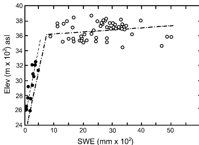
Fig. 4.24 The altitudinal gradient of winter precipitation (solid dots) determined from snow-course data and accumulation measured on glaciers in the Front Range, Colorado in 1970 expressed as snow water equivalent (from Alford, 1985).
