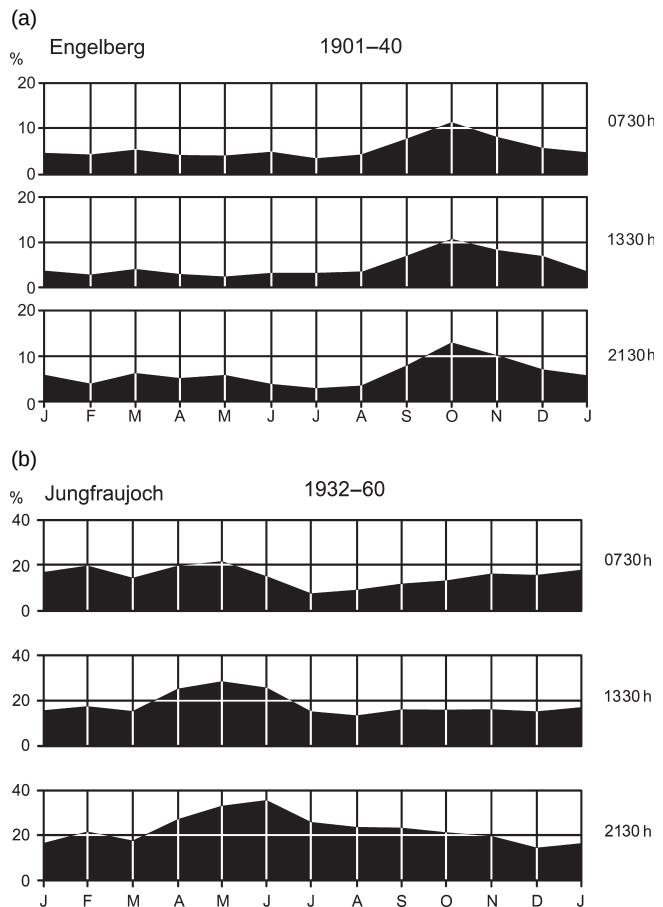
Fig. 5.17 Diurnal fog frequency on the Bernese Plateau (a) and on an alpine summit (b) (from Wanner, 1979).
