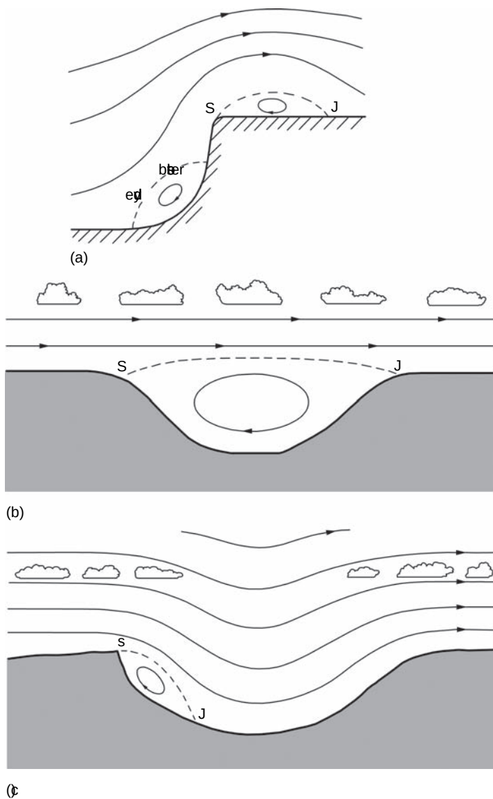
Fig. 2.32 Examples of flow separation: (a) separation at a cliff top (S), joining at J. A “bolster” eddy resulting from flow divergence is shown at the base of the steep windward slope; (b) separation on a lee slope with a valley eddy. The upper flow is unaffected; (c) separation with a small lee slope eddy. A deep valley may cause the air to sink resulting in cloud dissipation above it (from Scorer, 1978).
