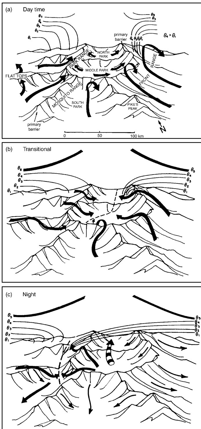
Fig. 3.48 Conceptual model of the regional-scale circulation system over the inter-montane basins of the Colorado Rocky Mountains. (a) Daytime inflow; (b) transition phase; (c) nocturnal outflow (from Bossert and Cotton, 1994).
