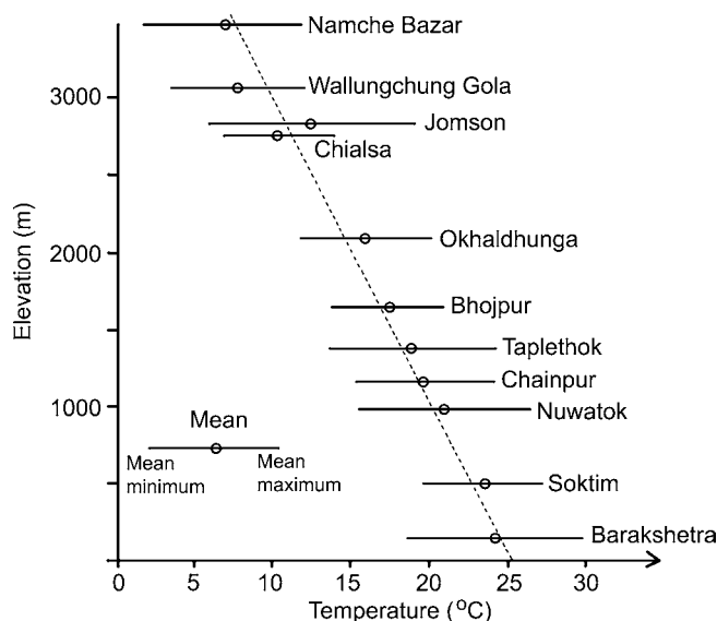
Fig. 5.6 The range of mean monthly temperatures versus altitude in the Nepal Himalaya (after Dobremez, 1976).
