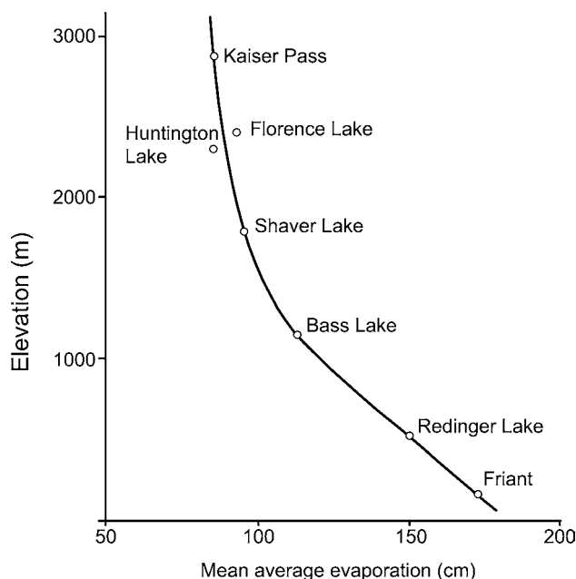
Fig. 4.38 Estimated annual evaporation (cm) from water surfaces in central California based on pan measurements and meteorological data (after Longacre and Blaney, 1962).
