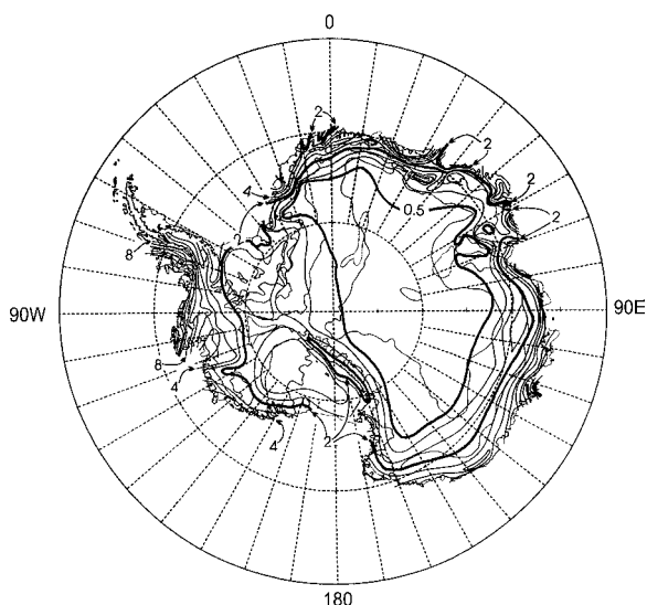
Fig. 5.27 Antarctic annual accumulation (cm) (from Bromwich and Parish, 1998).
