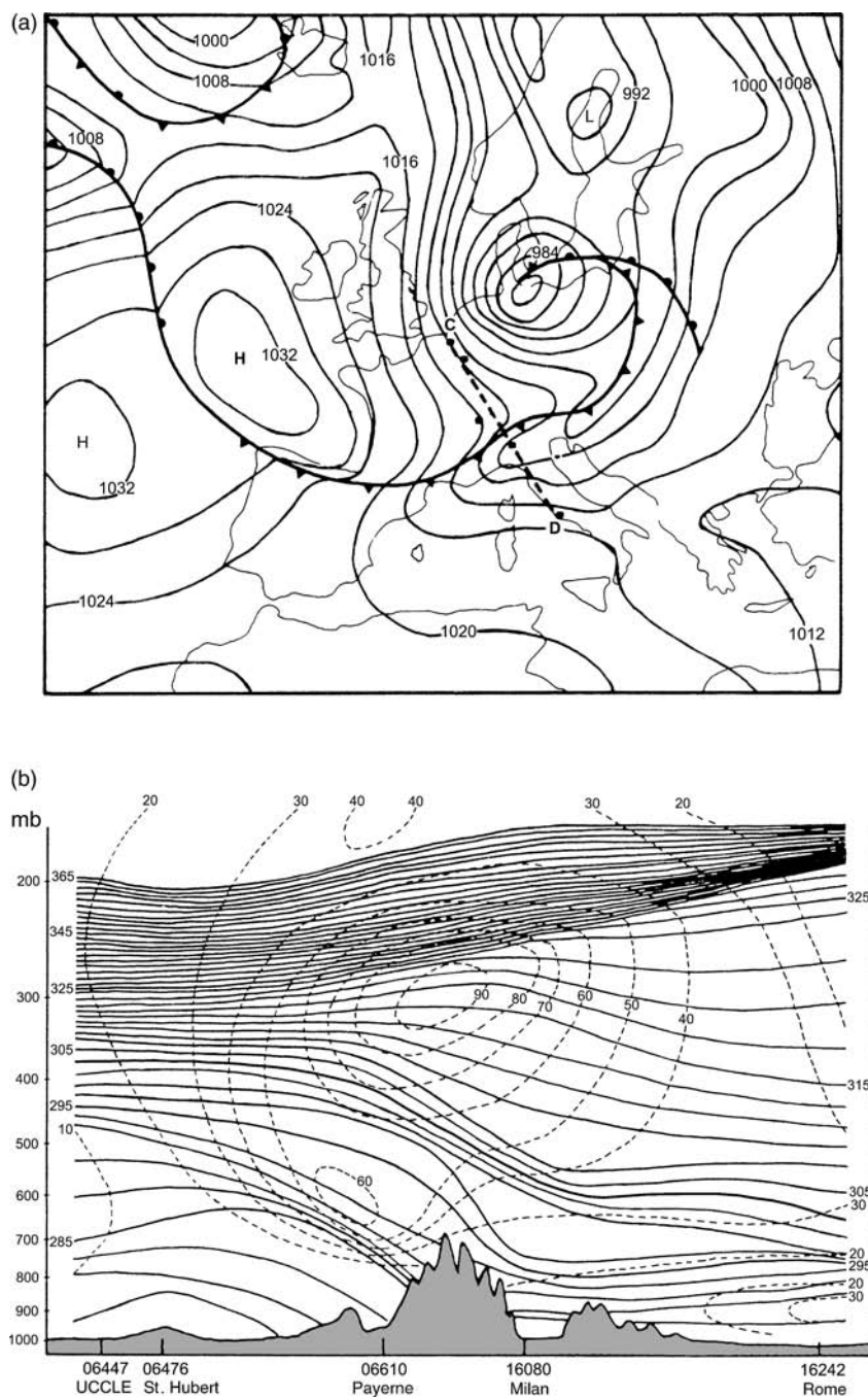
Fig. 3.13 Lee cyclogenesis associated with a frontal passage over the Alps. (a) Surface pressure map, 3 April 1973, 0000 GMT; (b) Cross-section along the line C-D of (a). Isentropes (K) and isotachs (knots); (c) As (a) for 1200 GMT; (d) As (b) for 1200 GMT along the line E-F (from Buzzi and Tibaldi, 1978).
