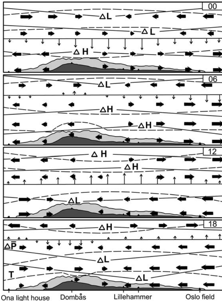
Fig. 3.35 Pressure anomalies (schematic) in relation to the mountain and valley wind system at 6-h intervals along the Gudbrandsdalen, Norway (after Sterten and Knudsen, 1961). Farder ( 59^\circ N) is at the mouth of Oslo Fjord, Ona ( 63^\circ N) is on the west coast. The land rises to 650 m at Dombås.
