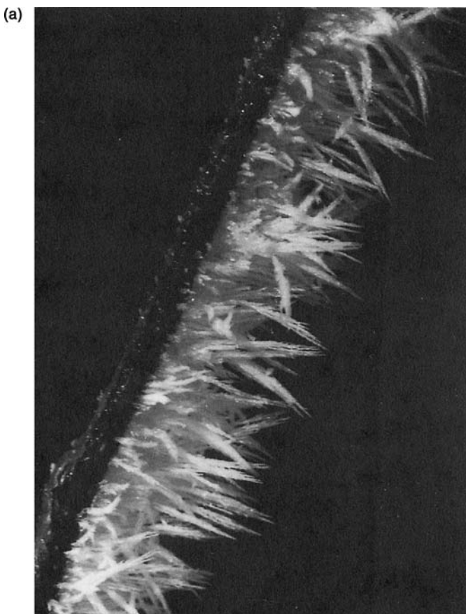
Fig. 4.33 (a) soft rime needles on a twig; the air temperature was -4^{\circ}\text{C} with 96 percent relative humidity in a light wind, 1030, 20 January 1953. (b) hard rime feathers on an anemometer support cable in a light, at -3^{\circ}\text{C} , 100 percent relative humidity, with occasional light drizzle and fog, 0900, 28 November 1953 (Hohenpeissenberg Observatory).
