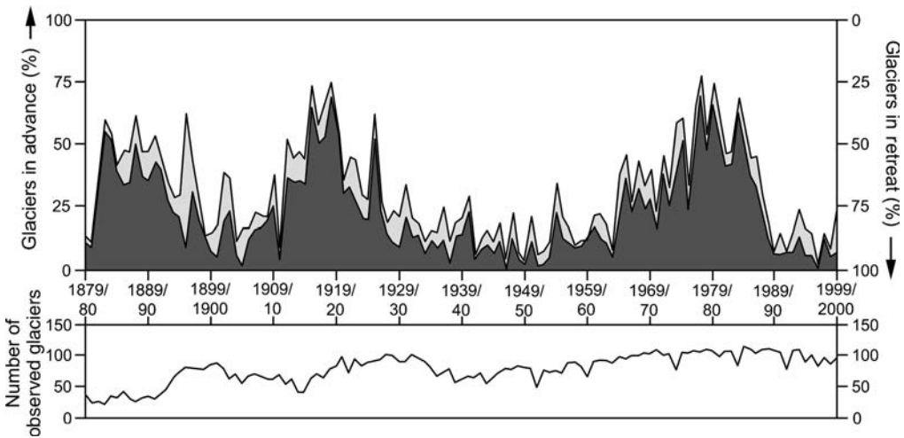
Fig 7.5 Percentage of Swiss glaciers showing advance (hatched) or retreat (white) of the terminus, 1879–80 to 1999–2000 (based on data provided by the World Glacier Monitoring Service, Zurich).
