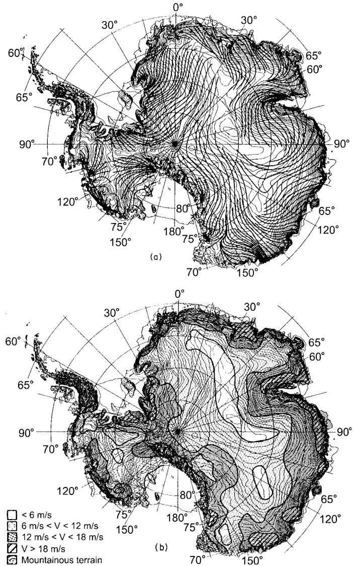
Fig. 5.26 Surface winds over Antarctica (from Parish and Bromwich, 1991).
