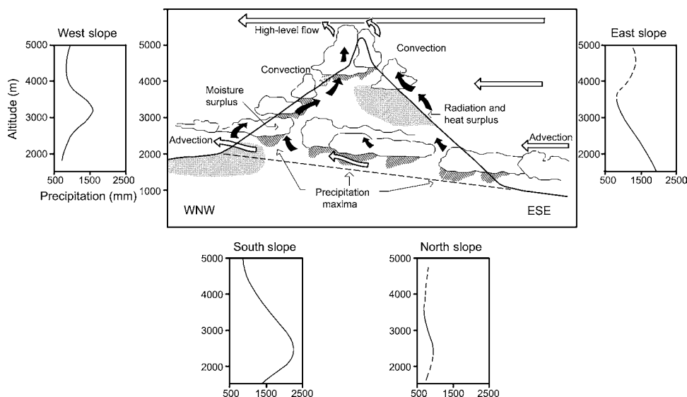
Fig. 5.2 Schematic view of daytime circulation, moisture advection, cloudiness and precipitation on Mt. Kenya (adapted from Winiger, 1981).
