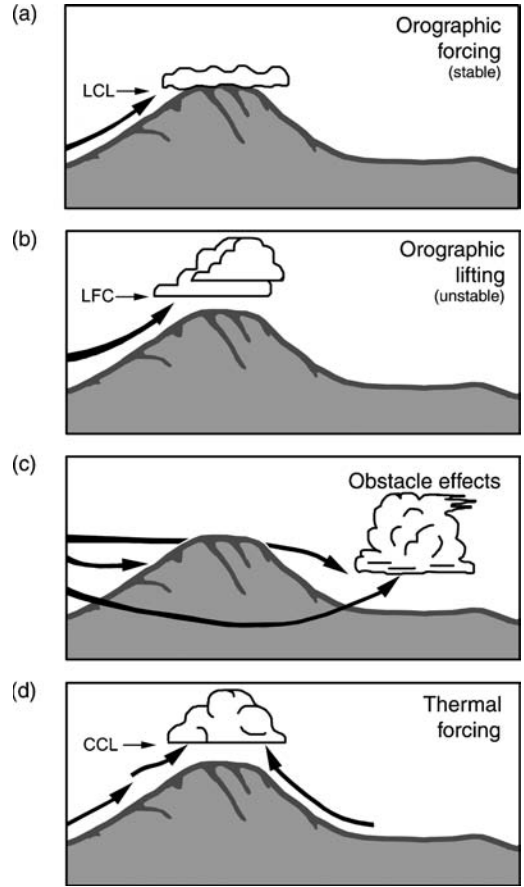
Fig. 4.9 Schematic illustration of the effects of a mountain barrier on cloud formation (modified after Banta, 1990).
