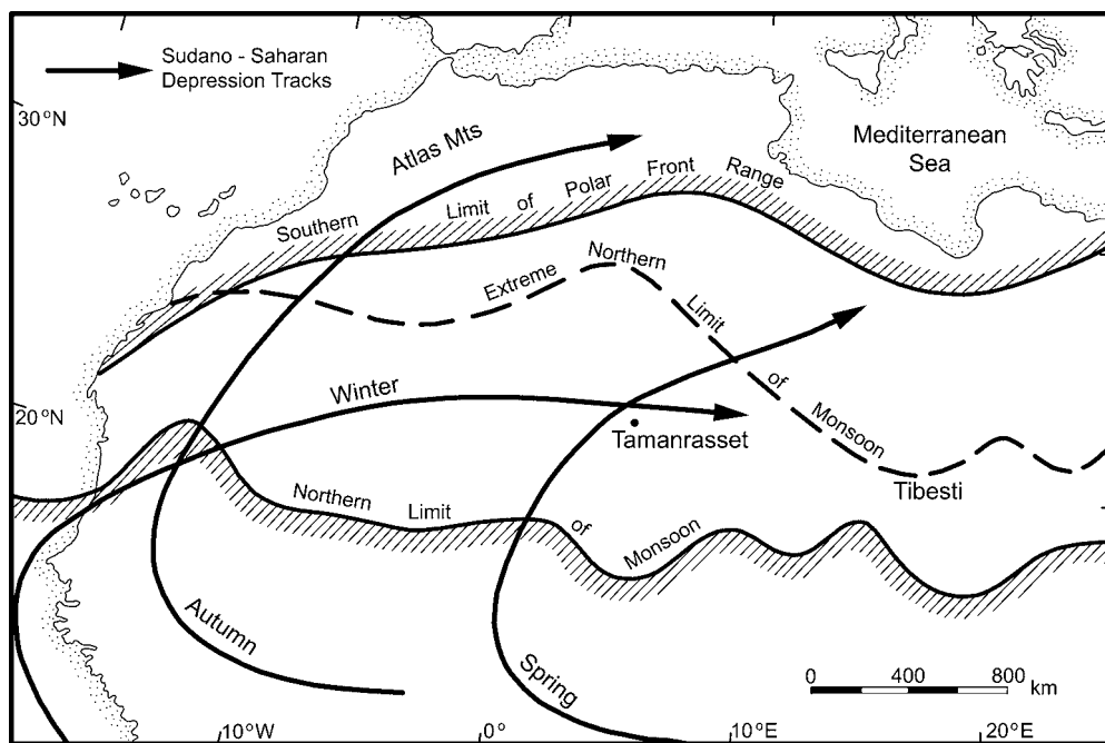
Fig. 5.8 Extent of precipitation systems affecting western and central North Africa and typical tracks of Sudano–Saharan depressions (after Dubief, 1962; Yacono, 1968).
