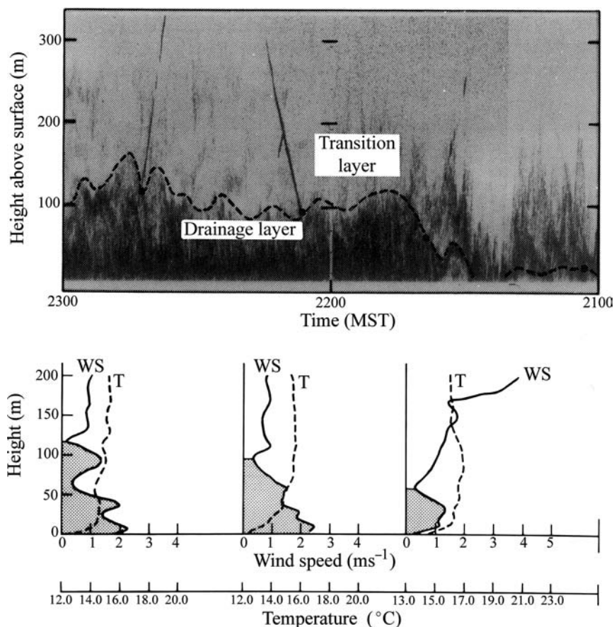
Fig. 3.42 Sodas returns (above) and tethersonde observations (below) during drainage initiation in Willy's Gulch, Colorado, 16 September 1986. The arrows denote the transit direction of the tethersonde balloons; the point at 2140 MST marks the start of northerly drainage flow, with a decrease of southerly ridge top winds from about 7 \text{ m s}^{-1} to 3\text{--}4 \text{ m s}^{-1} . The drainage layer thickens to \geq 100 \text{ m} (dashed line). Wind speed (WS) and temperature (T) profiles correspond to the three soundings on the sodar record; the drainage layer is stippled. Time runs from right to left (Neff and King, 1989, J. appl. Met. , 28, p. 522, Fig.5).
