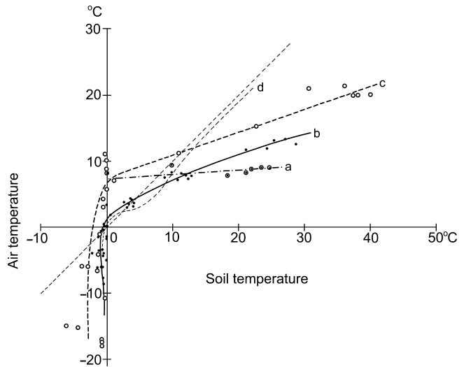
Fig. 2.38 Relations between monthly soil temperatures (0–1 cm) and air temperature (2 m) near the forest limit, Obergürl, Austria (2072 m), June 1954–July 1955 (Aulitsky, 1962, from Yoshino, 1975).
