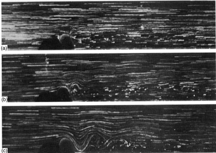
Fig. 3.20 Lee waves developed in simulated northwesterly flow over a model Alpine/Pyrenean topography. This laboratory experiment is similar to that of Figure 3.12. The sequence shows (a) no lee waves (b) upper level lee waves and (c) lee waves at all levels in response to increasing Froude number, F_0 . The transitions between (a) \rightarrow (b) and (b) \rightarrow (c) occur for F_0 = 0.25 and 0.37 , respectively; the equivalent atmospheric free stream winds are 8.6 \text{ m s}^{-1} and 12.8 \text{ m s}^{-1} (D. J. Boyer and Met. Atmos. Physics 1987, Springer).
