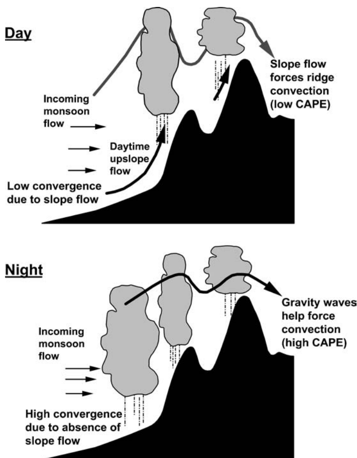
Fig. 5.3 Schematic illustration of nocturnal precipitation in the central Himalaya (from Barros and Lang, 2003). Convectively available potential energy.
