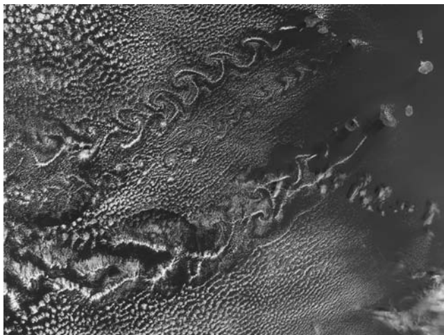
Fig. 3.23 Vortex street downstream of the Cape Verde Islands, 5 January 2005, as seen in MODIS bands 1, 3 and 4 (NASA-GSFC).
