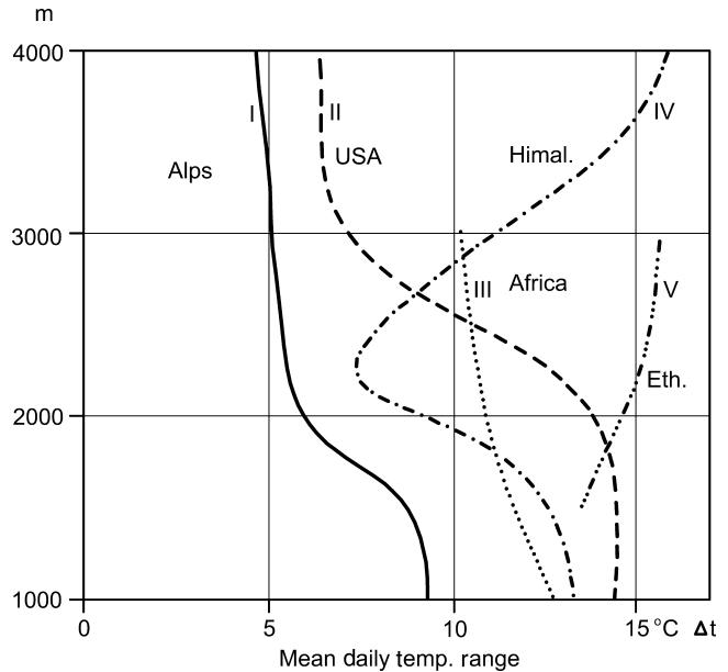
Fig. 2.18 Mean daily temperature range versus altitude in different mountain and highland areas: I, Alps; II, western USA; III, eastern Africa; IV, Himalaya; V, Ethiopian highlands (after Lauscher, 1966).
