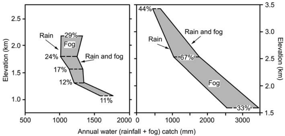
Fig. 4.32 Annual rainfall and fog catch versus elevation on Mauna Loa, Hawaii. Left: lee slope. Right: windward slope. The percentage increase in annual total due to fog catch is shown at the elevations of measurements (after Juvik and Ekern, 1978).
