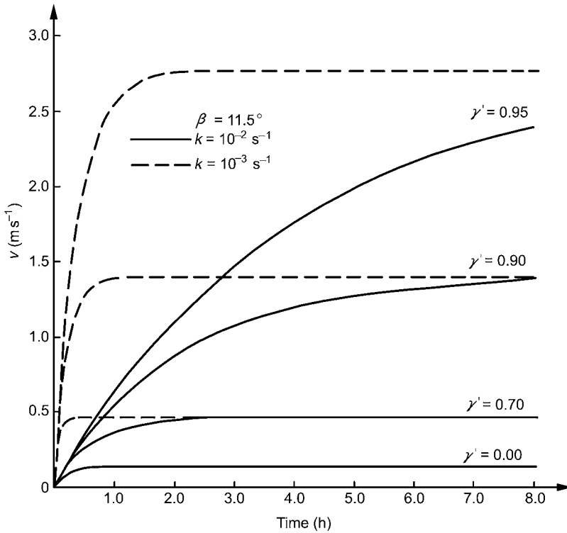
Fig. 3.34 Drainage wind velocity ( v ) on an 11.5^\circ slope as a function of time, for different values of lapse rate ( \gamma ) and friction coefficient ( k ) (from Petkovšek and Hočevar, 1971).
