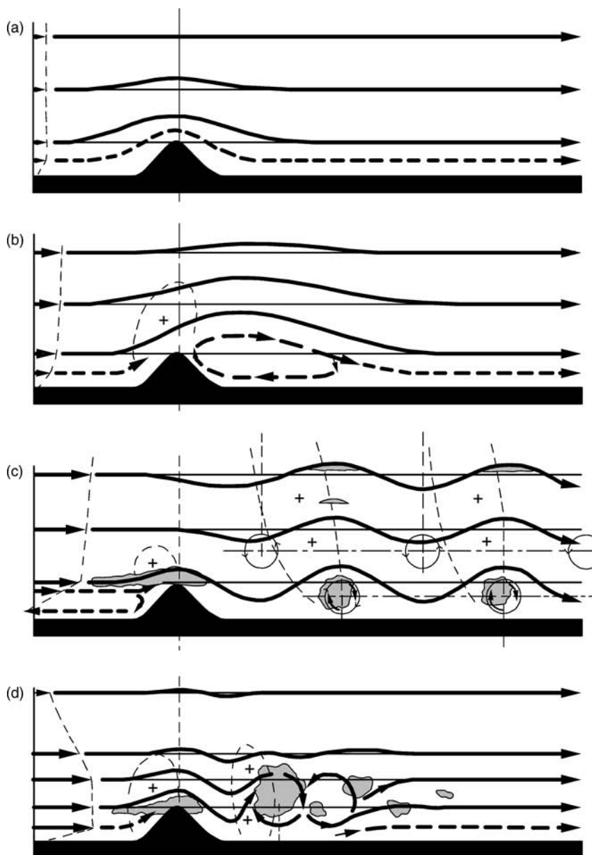
Fig. 3.14 Types of airflow over a mountain barrier in relation to the vertical profile of wind speed. (a) Laminar streaming; (b) Standing eddy streaming; (c) Wave streaming, with a crest cloud and downwind rotor clouds; (d) Rotor streaming (from Corby, 1954).
