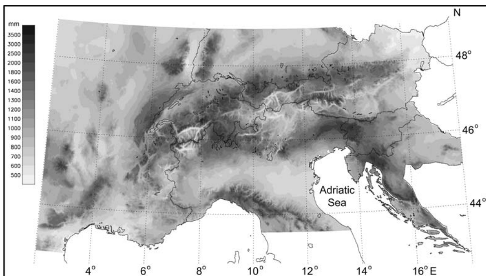
Fig. 5.14 Annual precipitation over the Alps for 1966–95 based on a dense station network (see text) (simplified after Frei and Schär, 1998).
