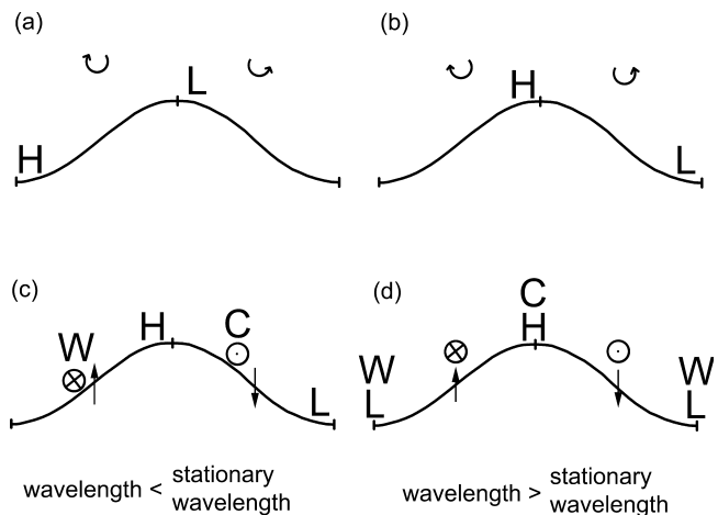
Fig. 3.1 Schematic vertical section illustrating the response of the atmosphere to westerly flow over a mountain range. (a) and (b) are barotropic atmospheres; the clockwise (counterclockwise) arrows indicate the generation of anticyclonic (cyclonic) vorticity for a northern hemisphere case. (c) and (d) are baroclinic atmospheres (from Hoskins and Karoly, 1981).
