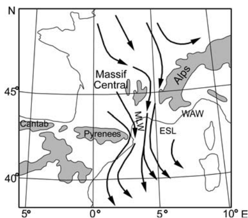
Fig. 3.6 “Corner effect” on airflow east of the Massif Central (the Mistral), east of the Pyrenees (the Tramontane), and east of the Cantabrian Mountains of Spain (partly after Cruette, 1976). ESL, eastern shear line of the Mistral; WAW, western Alps wake.
