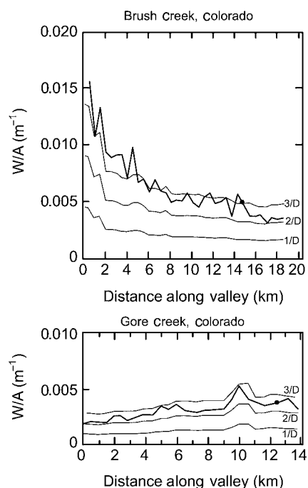
Fig. 3.41 Plots of valley width/area ( W/A ) ratios ( \text{m}^{-1} ) along Brush Creek, Colorado (draining) and Gore Creek, Colorado (pooling) (from Whiteman 1990, after McKee and O'Neal 1989).
