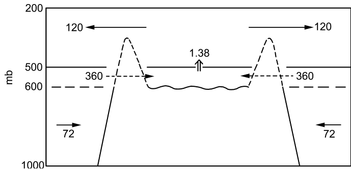
Fig. 2.22 Components of the mean daily thermal circulation ( \text{cm s}^{-1} ) above Tibet (from Flohn, 1974).
