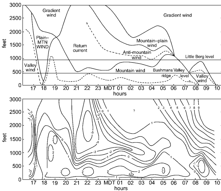
Fig. 3.47 Time section of local winds ( \text{m s}^{-1} ) in and above Bushmans Valley, Drakensberg Mountains, 12–13 March 1965 (from Tyson, 1968b).
