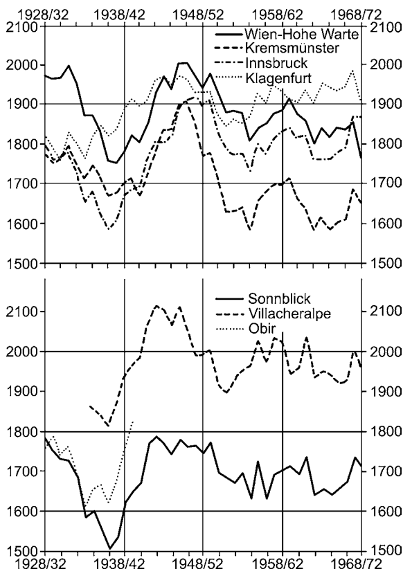
Fig 7.2 Changes from 1928–32 to 1968–72 in annual totals of sunshine hours at four stations in the Austrian lowlands (above) and at three mountain stations (below), plotted as a 5-year moving average (from Steinhauser, 1973).
