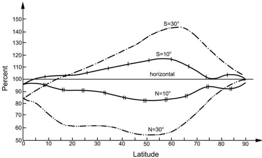
Fig. 2.35 Annual totals of possible direct solar radiation according to latitude for 10° and 30° north- and south-facing slopes, in percentages relative to those for a horizontal surface (from Kondratyev and Federova, 1977).
