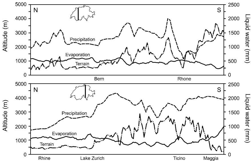
Fig. 5.16 North-south transects of precipitation for 1971–90 and actual evaporation for 1973–92 across the Swiss Alps (after Spreafico and Weingartner, 2005).
