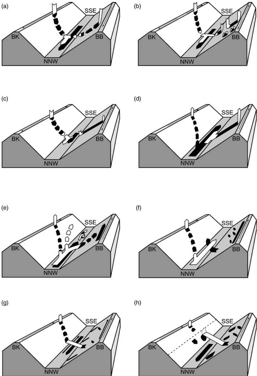
Fig. 3.40 Model of mountain and valley wind system in the Dischma Valley, Switzerland. (a) Midnight to sunrise on the east-facing slope; (b) sunrise on the upper east-facing slope; (c) whole facing slope in sunlight; (d) whole valley in sunlight; onset of valley wind; (e) west-facing slope receiving more solar radiation than east-facing slope; (f) solar radiation only tangential to east-facing slope; (g) sunset on east-facing slope and valley floor; (h) after sunset on the lower west-facing slope (from Urfer-Henneberger, 1970).
