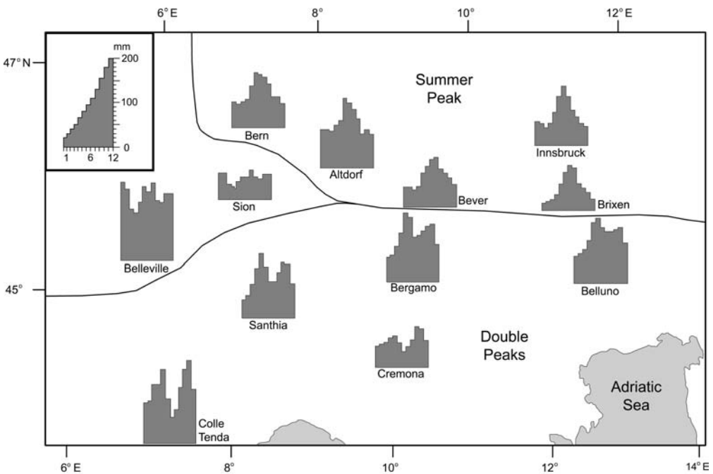
The annual cycle of precipitation in the Alps (1931-1960)
