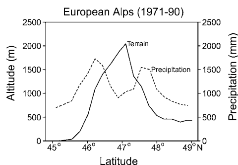
Fig. 5.15 Mean annual precipitation (dashed) and elevation (solid line) for a south–north transect through the eastern Alps between the Gulf of Venice and Bavaria (based on Schwarb et al. , 2001).
