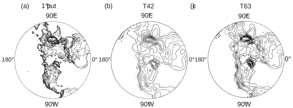
Fig. 3.2 The representation of northern hemisphere topography in 1^\circ resolution data and in spectral models with triangular truncation at T42 and T63 (from Hoskins, 1980).
