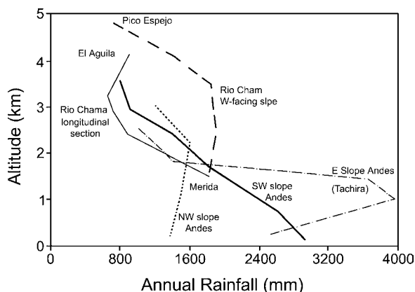
Fig. 5.29 Precipitation versus elevation on different slopes of the Venezuelan Andes (from Pulwarty et al. , 1998).
