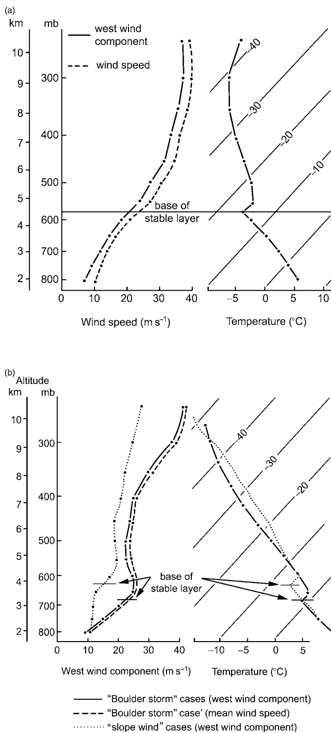
Fig. 3.30 Composite soundings for times of windstorms in Boulder, Colorado. (a) Upwind sounding (west of the Continental Divide). (b) Downwind soundings (Denver) for storms in Boulder or on the slopes just to the west (from Brinkmann, 1974a).
