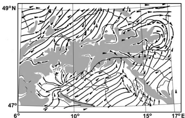
Fig. 3.7 An example of a streamline analysis for the Alps, omitting areas exceeding 750 m altitude, 24 June 1978 (from Steinacker, 1981).
