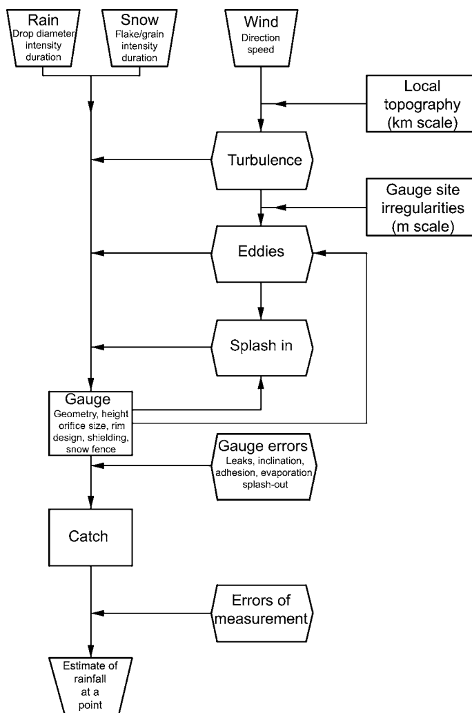
Fig. 4.29 Schematic summary of processes and problems involved in the determination of rain gauge catch (after Rodda, 1967).
