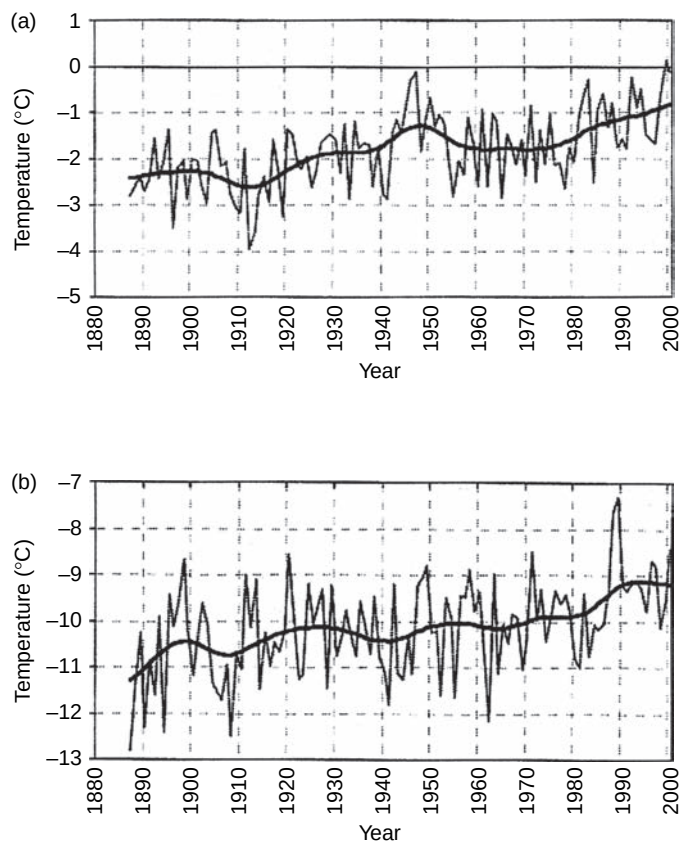
Fig 7.1 Time series of (a) summer half-year and (b) winter half-year air temperatures ( ^{\circ}\text{C} ) at Sonnblick Observatory, 1887–2000 (after Auer et al. , 2000). (Courtesy Zentralanstalt für Meteorologie und Geodynamik, Vienna.)
