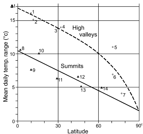
Fig. 2.3 Mean daily temperature range versus latitude for a number of high valley and summit stations (after Lauscher, 1966).
