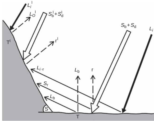
Fig. 2.37 Components of solar and infrared radiation incident on slopes.
