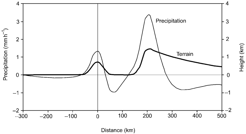
Fig. 4.28 Precipitation rate ( \text{mm h}^{-1} ) for idealized terrain heights (km) in western Oregon according to the linear theory of Smith and Barstad (2004) (from Smith et al. , 2005).
