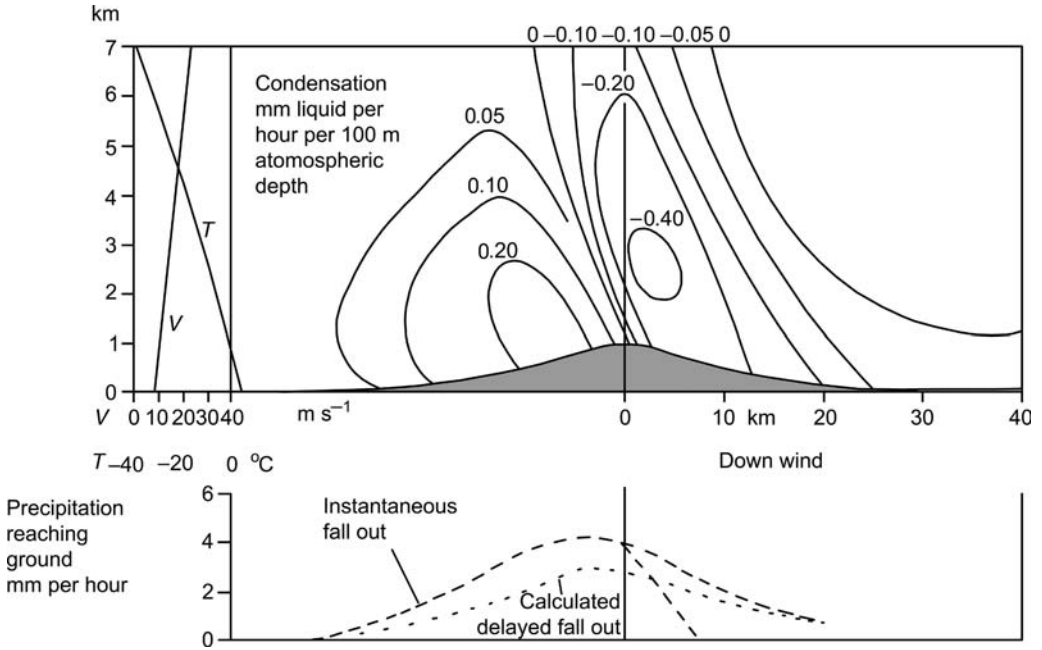
Fig. 4.26 Calculated condensation and precipitation ( \text{mm h}^{-1} ) for the airflow case shown in Figure 4.25 (b) (from Walker, 1961).
