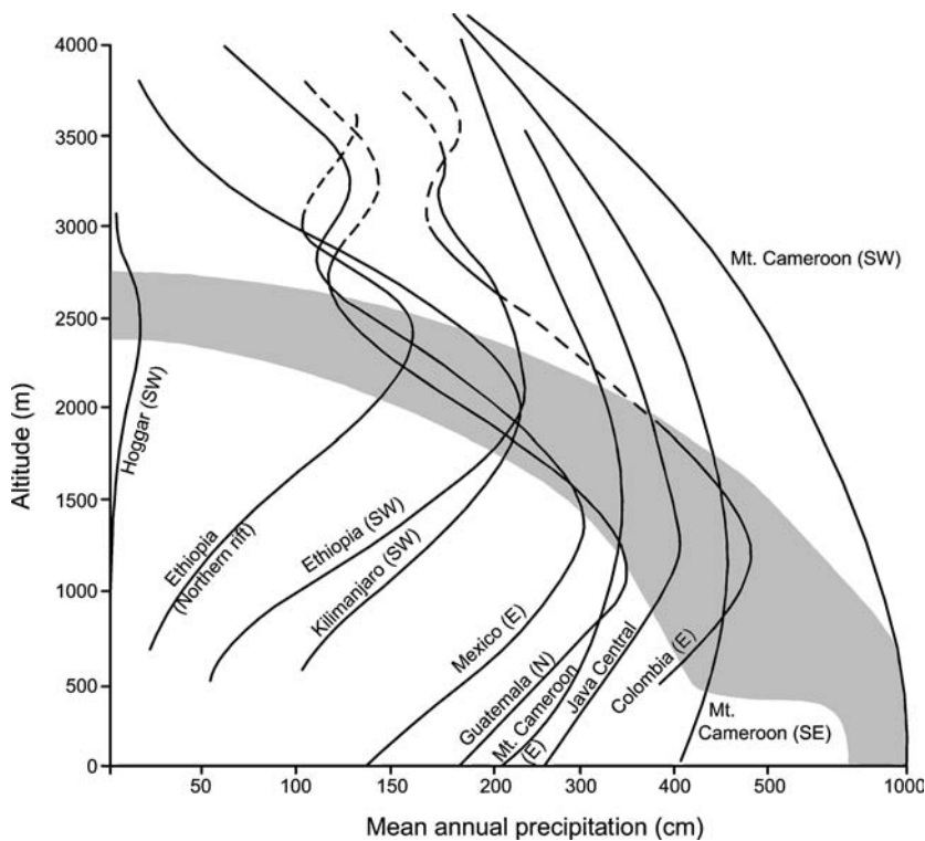
Fig. 4.18 Generalized profiles of mean annual precipitation (cm) versus altitude in the tropics (from Lauer, 1975). The shading denotes the zone of maximum precipitation.
