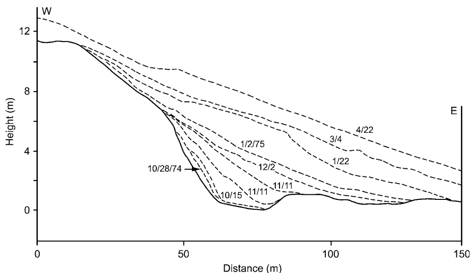
Fig. 4.36 Snow drift accumulation, 1974–5 at a site on Niwot ridge, Colorado (3450 m) (after Berg and Caine, 1975). Winds are predominantly downslope from the west.
