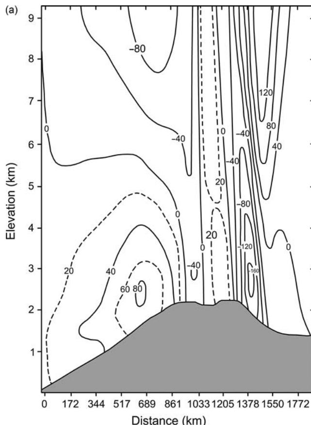
Fig. 4.27 Model simulations for a storm with a westerly airflow over northern California, 21–23 December 1964: (a) computed steady-state vertical motion field ( \text{cm s}^{-1} ); (b) computed precipitation rate (solid line) and observed values (dots) (from Colton, 1976).
