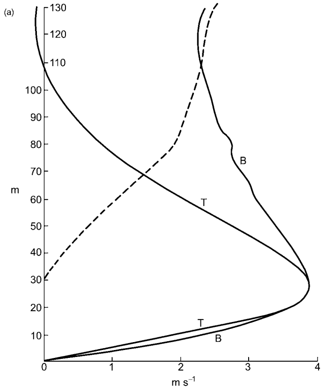
Fig. 3.33 Pilot balloon observations (B) and theoretical (T) slope winds on the Nordkette, Innsbruck: (a) upslope; (b) downslope (from defant 1949). The dashed lines show the differences between theory and observation.
