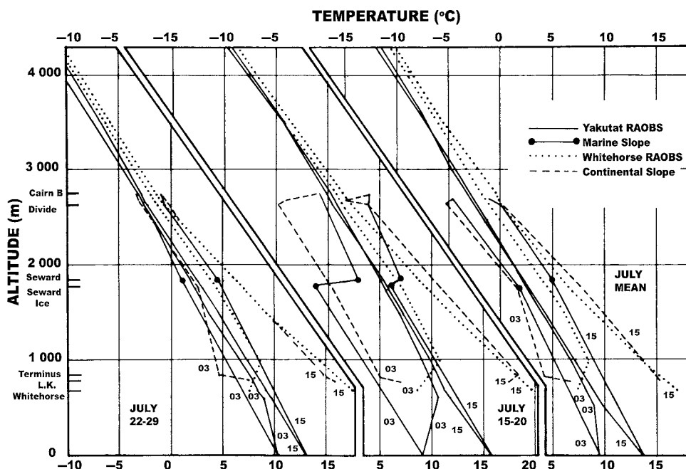
Fig. 5.22 Temperature soundings at Yakutat and Whitehorse and lapse rates in the St. Elias region, July 1964 (from Marcus, 1965).
