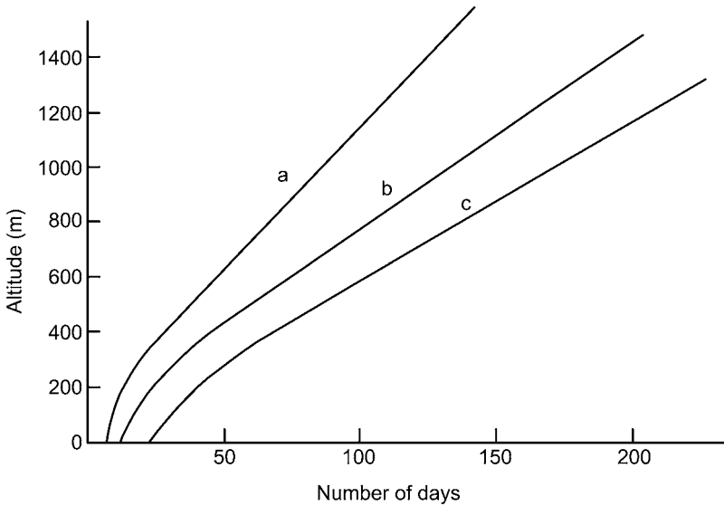
Fig. 4.22 The average number of days with snow lying versus altitude on various mountains in Great Britain: (a) an average mountain in the west of Great Britain; (b) an average mountain in the whole of Great Britain; (c) an average mountain in central Scotland (from Jackson, 1978).
