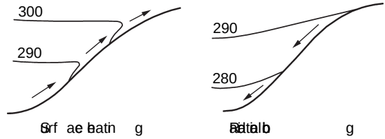
Fig. 2.25 Schematic isentropes on slopes during surface heating and radiative cooling (after Cramer and Lynott, 1961).
