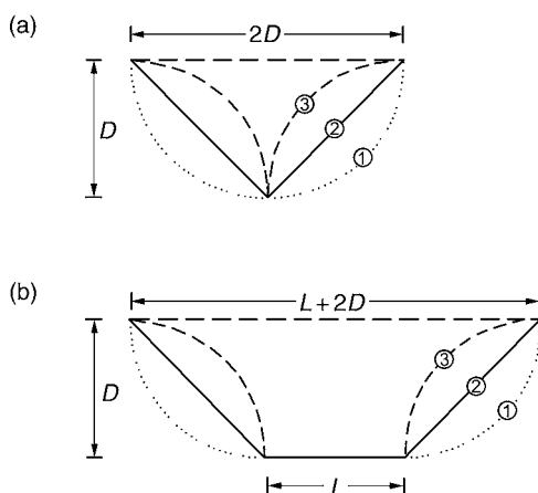
Fig. 3.36 Depth–width and shape relationships in idealized valley cross-sections for a valley without and with a horizontal floor. See text (Müller and Whiteman, 1988).
