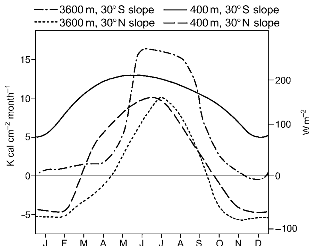
Fig. 4.3 Calculated net radiation on north- and south-facing slopes of 30° in the Caucasus at 400 m and 3600 m (based on Borzenkova, 1967).
