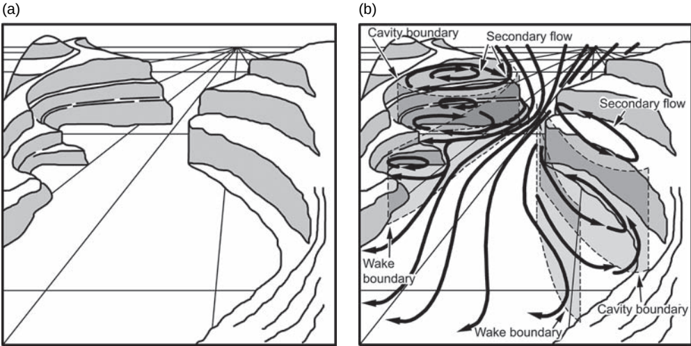
Fig. 6.4 Schematic model of turbulent wake effects associated with airflow along a canyon: (a) oblique view of canyon; (b) airflow along the canyon (from Start et al. , 1975).
