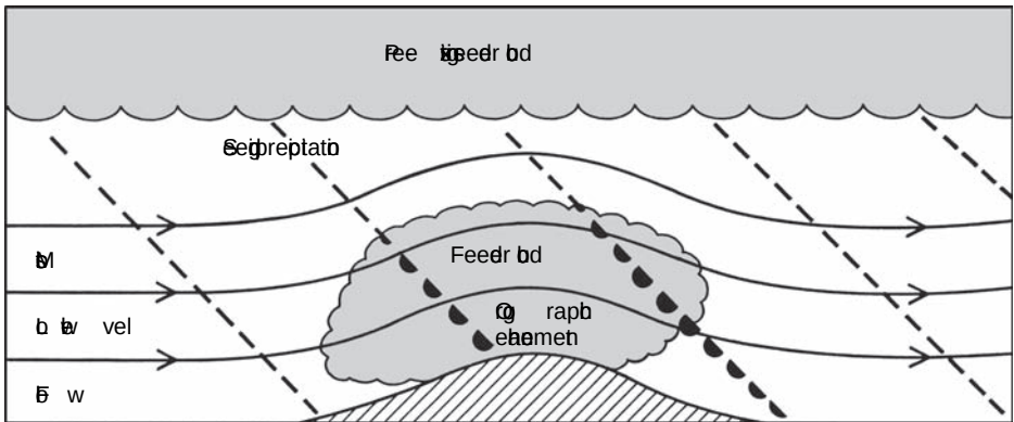
Fig. 4.14 Schematic illustration of seeder–feeder clouds and enhancement of precipitation over a hill (from Browning and Hill, 1981).
