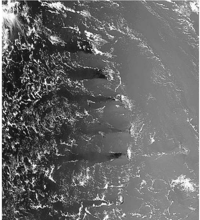
Fig. 3.25 Wakes in the lee of the Windward Islands of the Lesser Antilles (NASA Visible Earth).
