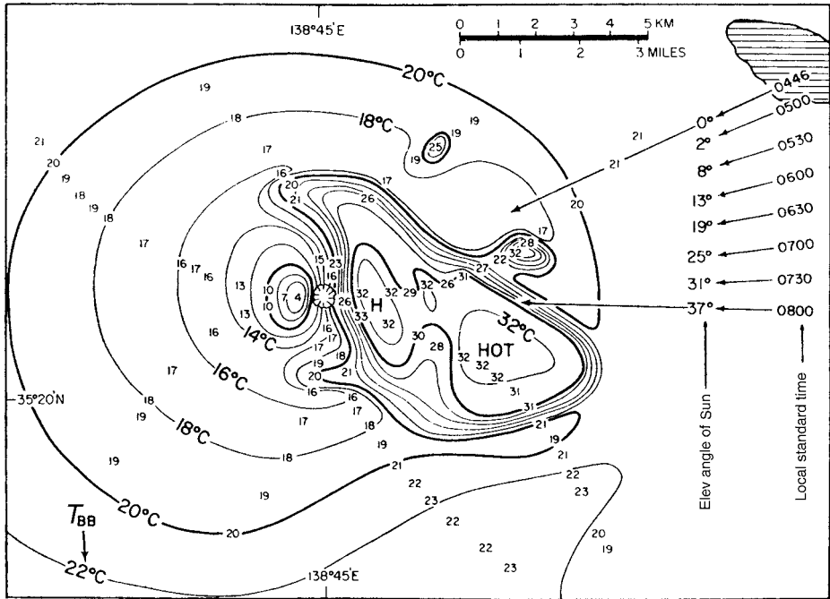
Fig. 4.6 Equivalent black-body temperatures ( T_{BB} ) measured by radiation thermometer from an aircraft over Mt. Fuji, 0743–0756 JGT, 28 July 1967. Solar altitude and azimuth is shown since sunrise (from Fujita et al. , 1968).
