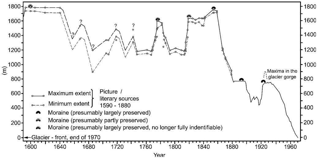
Fig 7.4 Variations in the front of the Lower Grindelwald Glacier, Switzerland, 1590–1970, relative to the 1970 terminal position (after Messerli et al. , 1978).
