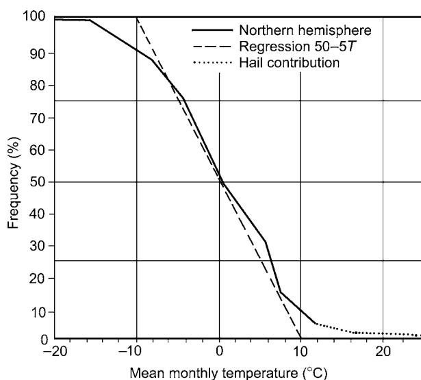
Fig. 4.21 Empirical relationship between monthly mean temperature ( ^\circ\text{C} ) and annual percentage frequency of solid precipitation in the northern hemisphere compared with the regression (50–5T) (from Lauscher, 1976b).
