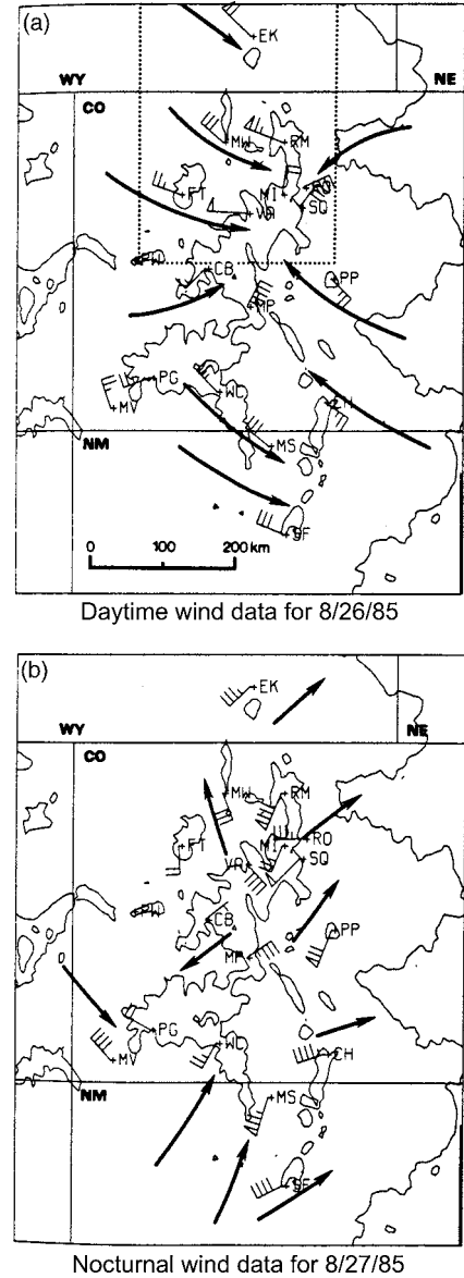
Fig. 3.45 Regional-scale diurnal wind reversals over the Rocky Mountains, Colorado, based on mountain-top observations of average resultant wind from (a) 1200 to 1500 MST for 26 August 1985 and (b) 0001 to 0300 MST for 27 August 1985 (from Bossert et al. , 1989).
