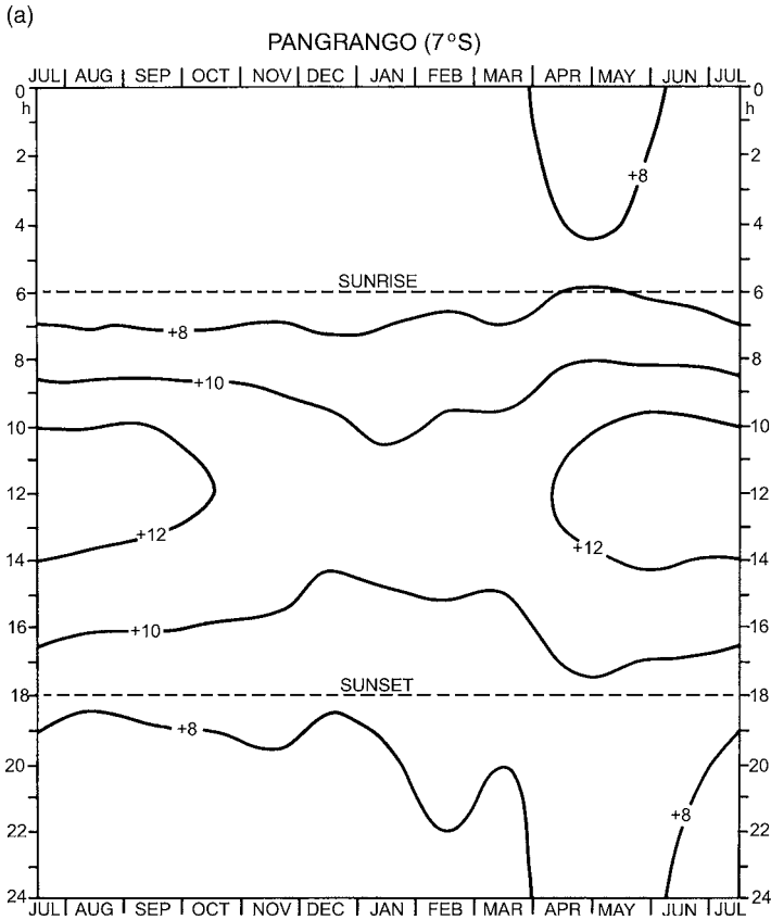
Fig. 2.2 Thermoisopleth diagrams of mean hourly temperatures (°C) at (a) Pangrango, Java, 7° S, 3022 m (after Troll, 1964) and (b) Zugspitze, Germany, 47° N, 2962 m (after Hauer, 1950).
