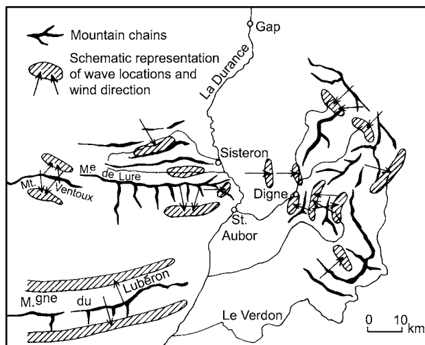
Fig. 3.22 Lee wave locations in relation to wind direction in the French Alps (after Gerbier and Béranger, 1961).
