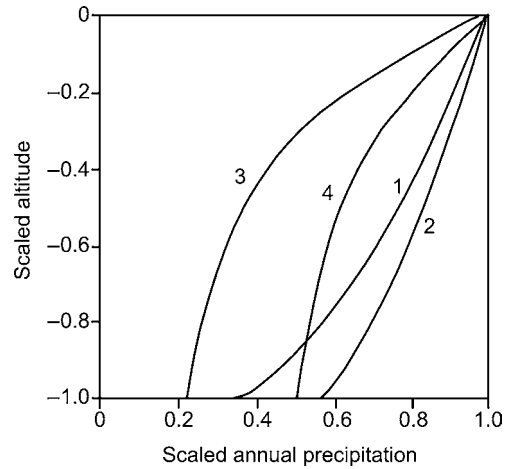
Fig. 5.9 Vertical gradients of annual precipitation in the Tien Shan and Pamir ranges. The values are scaled relative to the annual totals at the equilibrium line altitude (ELA) as estimated from the climatic snow line (adapted from Getker and Shchetinnikov, 1992). Zones 1 and 2 have spring–summer maxima in peripheral basins and interior basins, respectively. Zones 3 and 4 have winter–spring maxima in the corresponding topographic locations.
