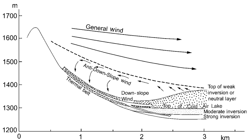
Fig. 4.7 Model of the thermal belt and cold air drainage on a mountain slope in central Japan (from Yoshino, 1984).
