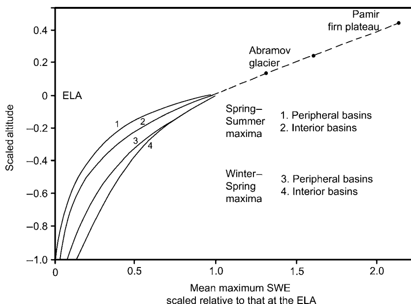
Fig. 5.10 Typical vertical gradients of maximum snow water equivalent (SWE) on macro-scale slopes in the Tien Shan and Pamir ranges (adapted from Getker, 1985).
