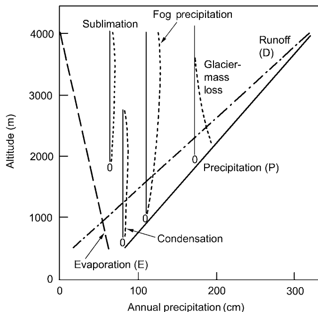
Fig. 4.39 Altitudinal profiles of mean annual precipitation (P), evaporation (E) and runoff (D) for the Swiss Alps (after Baumgartner et al. , 1983). The plots of condensation, sublimation, fog precipitation and glacier mass loss are offset on the abscissa for clarity.
