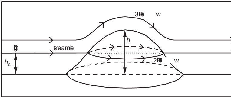
Fig. 2.28 Schematic illustration of a “dividing streamline” in stably-stratified airflow encountering a hill (modified after Etling, 1989).
