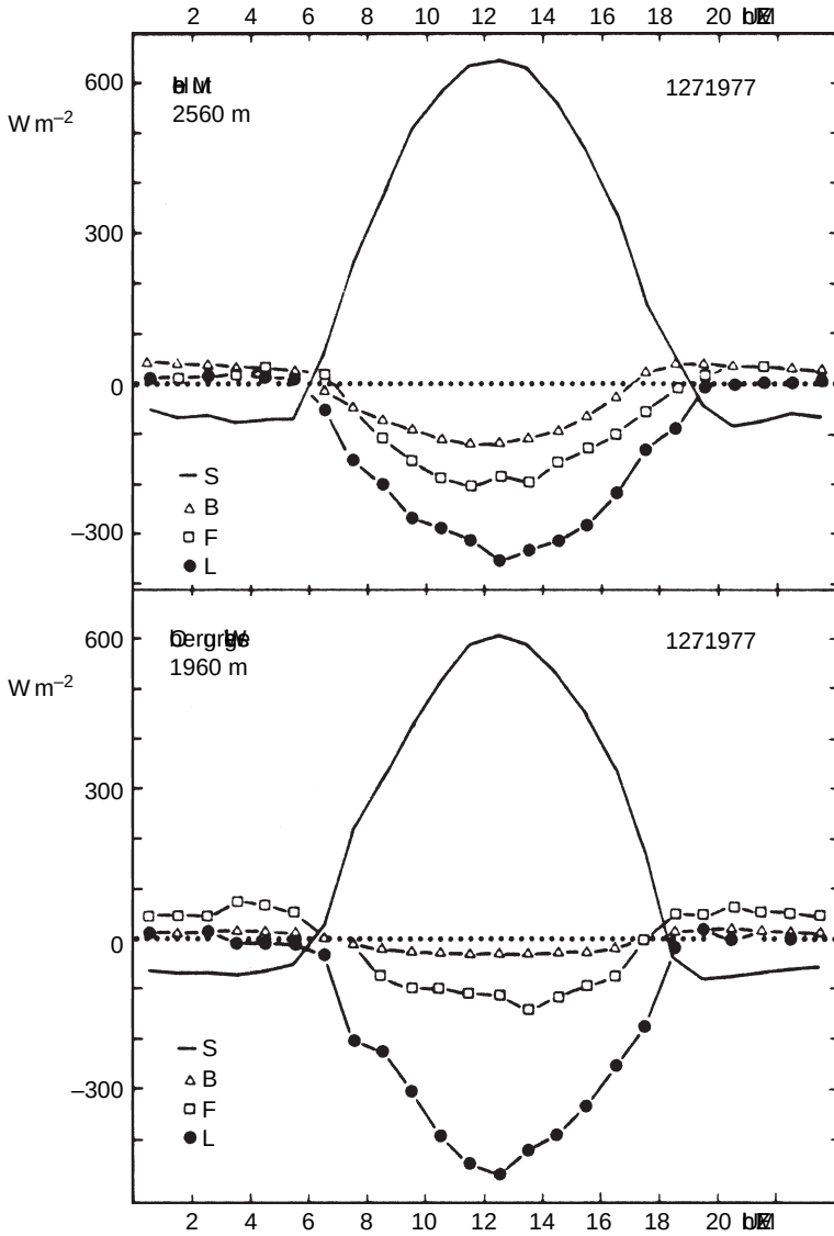
Fig. 4.2 Hourly values of energy budget components in the Austrian Tyrol, 12 July 1977, at Obergürgl-Wiese (1960 m) and Hohe Mut (2560 m) (from Rott, 1979).
