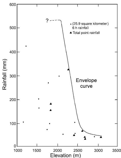
Fig. 5.20 The relation between precipitation and elevation for large storms in Colorado (after Jarrett, 1990). Source: Geomorphology 3(2), 1990, R. D. Jarrett, p. 184, Figure 5. Elsevier, Amsterdam.
