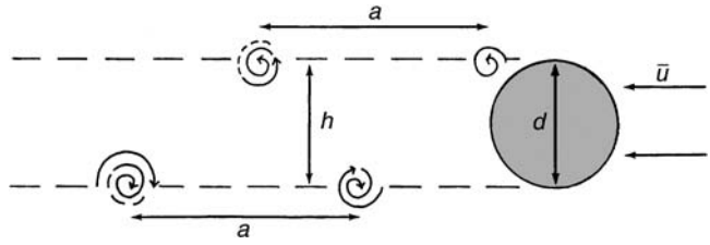
Fig. 3.24 Schematic illustration of a von Karman vortex in the lee of a cylindrical obstacle (after Chopra, 1973). d = obstacle diameter; h = lateral street width; a = longitudinal spacing between successive vortices in each row. Empirically, 0.3 < h/a < 0.5 .
