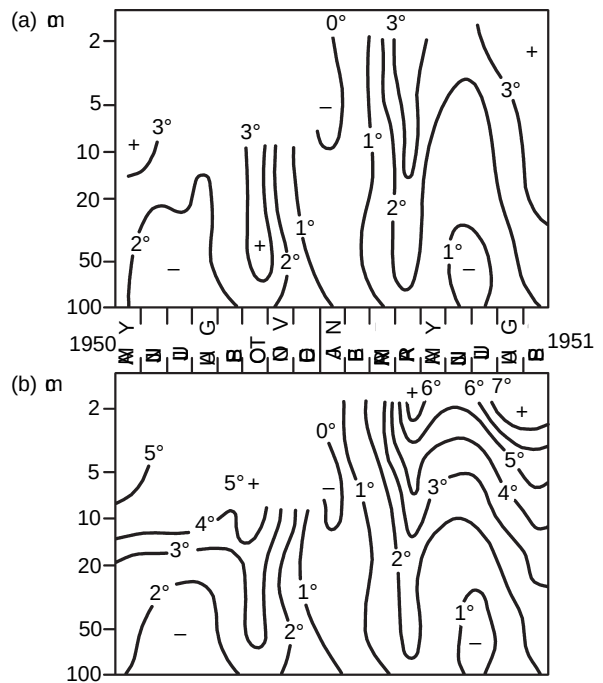
Fig. 2.42 Differences in monthly mean ground temperatures, south slope minus north slope, May 1950–September 1951 at Hohenpeissenberg, Bavaria. Daily means (a) and means at 1400 h (b) (after Grunow, 1952).
