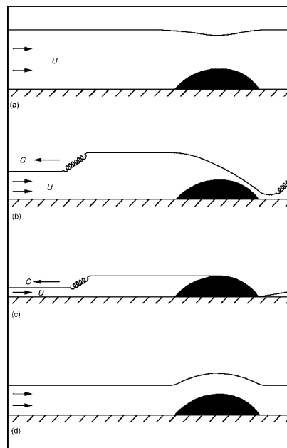
Fig. 3.19 Schematic illustrations of water flow over an obstacle in a channel. (a) Absolutely subcritical flow; (b) partially blocked flow with a bore progressing upstream at velocity c and a hydraulic jump in the lee; (c) totally blocked flow; (d) absolutely supercritical flow (from Long, 1969).
