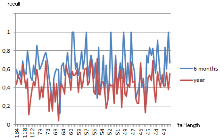
Fig. 5. Recall difference for entities with long “tails” after 6 month and a year of database population, shown on the x axis is the tail's length. we can see recall values for long-tail entities computed for their mentions in July and for mentions in December, where \text{recall} = \frac{\text{number of identified entities}}{\text{number of matching strings (both found and missing/unresolved entities)}} .
