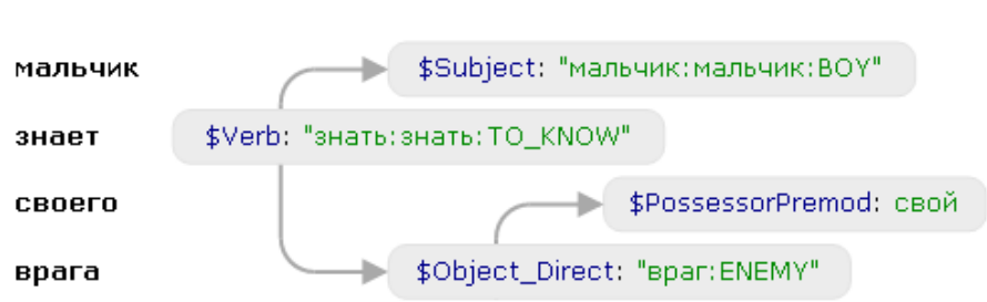
Fig. 3. Syntactic tree without non-tree links
