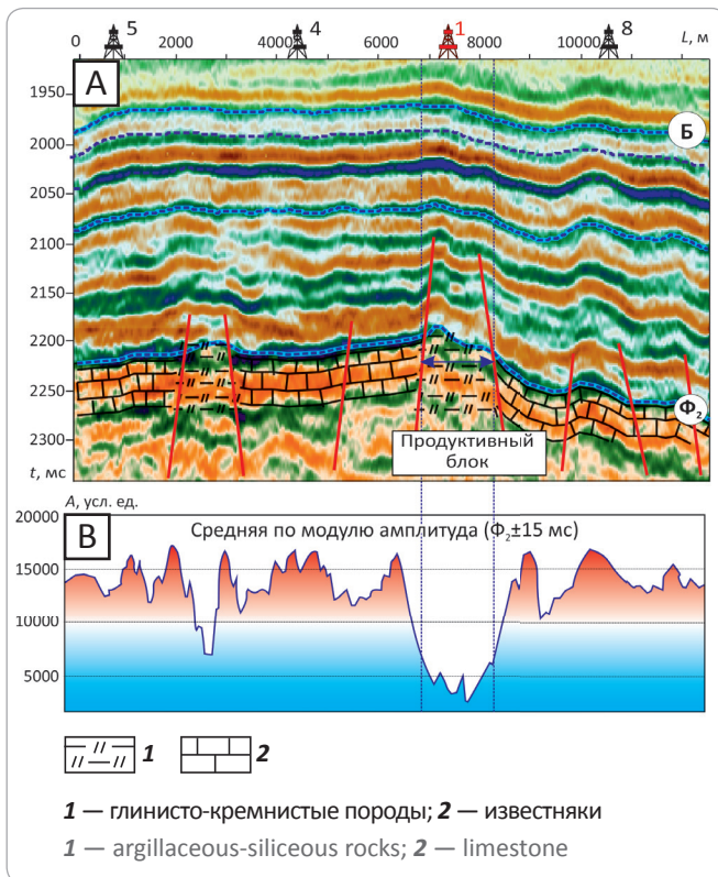
Fig. 5. Seismic time section along the Line 139425 (A) and diagram of reflection horizon \Phi_2 amplitudes (B), Vostochnoe field
