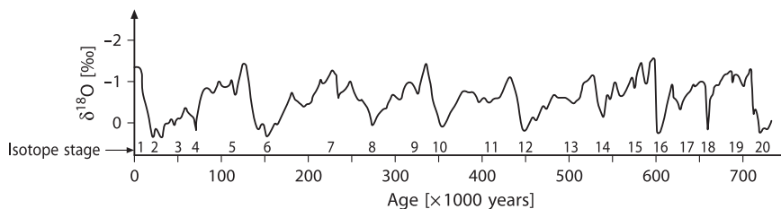
Fig. 3.48 Composite \delta^{18}\text{O} fluctuations in the foraminifera species G. sacculifer from Caribbean cores (Emiliani, 1966)
