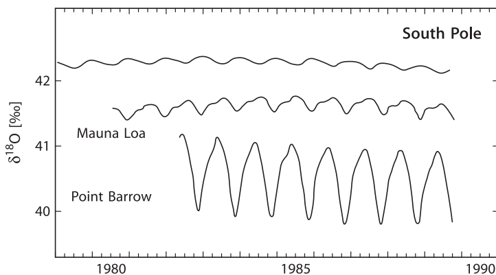
Fig. 3.32 \delta^{18}\text{O} seasonal record of atmospheric \text{CO}_2 from three stations: Point Barrow 71.3^\circ\text{N} , Mauna Loa 19.5^\circ\text{S} , South Pole 90.0^\circ\text{S} . (after Ciais et al., 1998)
