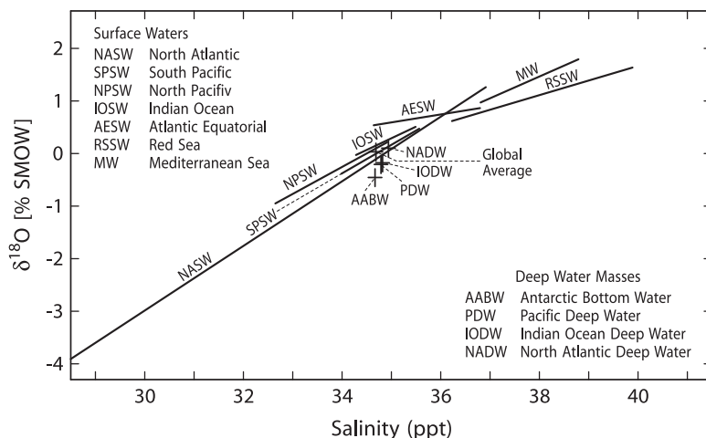
Fig. 3.18 Salinity vs \delta^{18}\text{O} relationships in modern ocean surface and deep waters (after Railsback et al. 1989)
