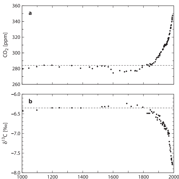
Fig. 3.33 Law Dome ice core CO 2 and \delta^{13}\text{C} record for the last 1000 years (after Trudinger et al. 1999)
