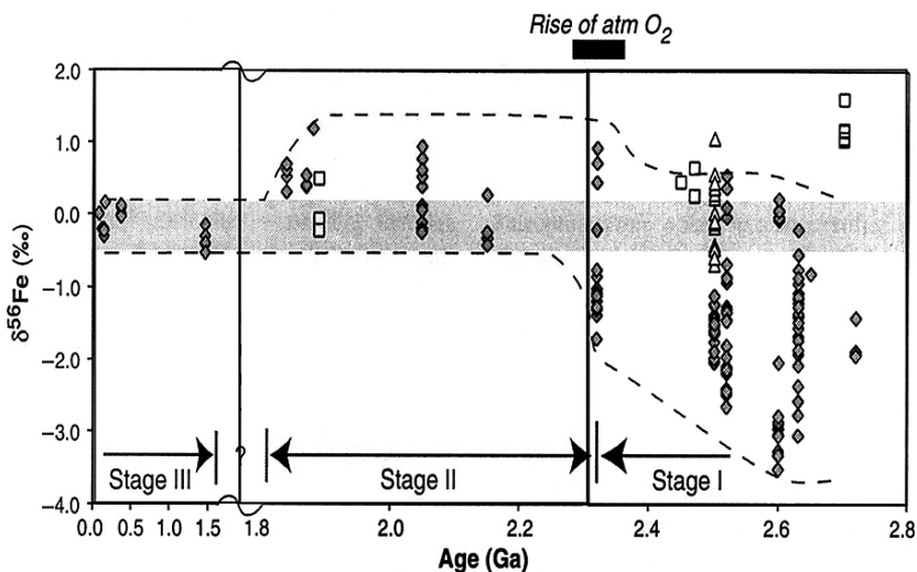
Fig. 3.28 \delta^{56}\text{Fe} values of pyrite and Fe oxides vs time showing three evolutionary stages of the ocean (Anbar and Rouxel (2007))
