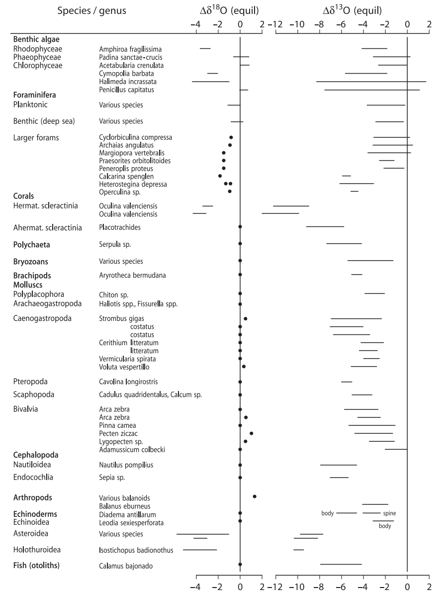
Fig. 3.42 \Delta\delta^{18}\text{O} and \Delta\delta^{13}\text{C} differences from equilibrium isotope composition of extant calcareous species (after Wefer and Berger, 1991)
