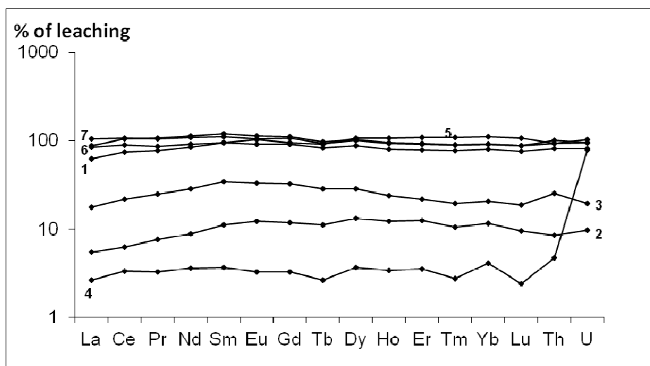
Figure 1. Results of REE , Th and U leaching (in % from total content) from lovozerite lujavrite (Lovozero massif, Kola Peninsula) with solutions: 1 – HCl, 2 – ammonium oxalate; 3 – trilon B, 4 - ammonium difluoride, 5 – HCl+ammonium oxalate, 6 - HCl+ trilon B, 7 - HCl+ammonium difluoride. ICP MS data.
