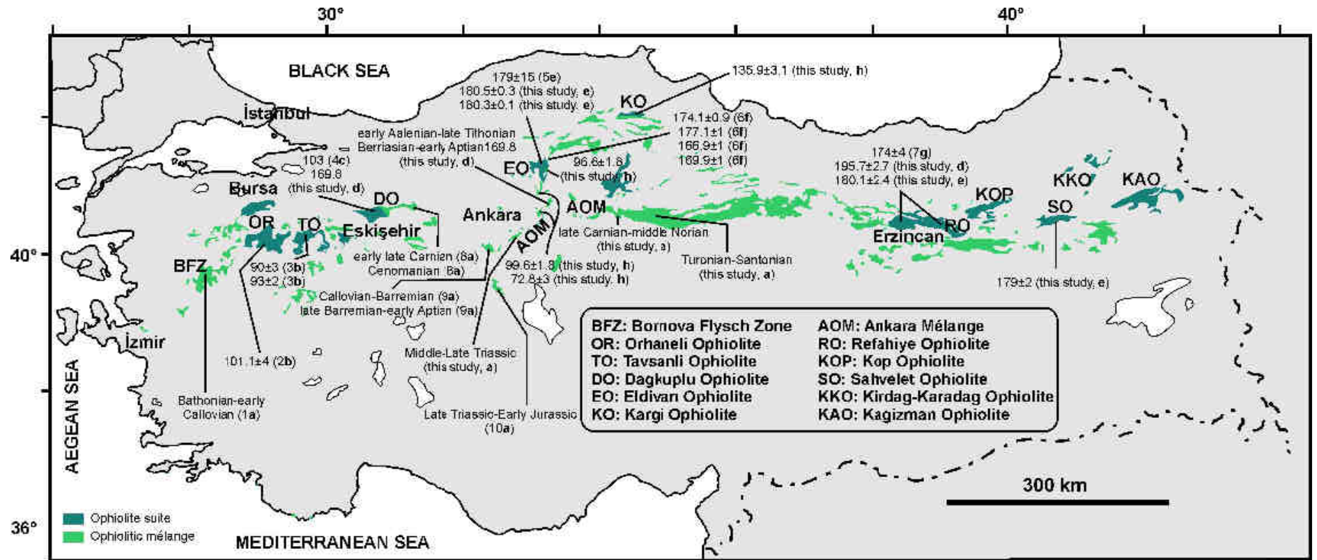
(1) Tekin & Gönçüoğlu (2009), (2) Harris et al. (1994), (3) Onen & Hall (2000), (4) Sarıfakıoğlu et al. (2009), (5) Dilek & Thy (2006), (6) Çelik et al. (2011), (7) Topuz et al. (2013), (8) Gönçüoğlu et al. (2001, 2010), (9) Rojay et al. (2004), (10) Uğuz et al. (1999) (a) Paleontological data, (b) ^{40}\text{Ar}/^{39}\text{Ar} amphibole ages from metamorphic sole, (c) Sm-Nd garnet ages from metamorphic sole, (d) ^{40}\text{Ar}/^{39}\text{Ar} hornblende ages from pegmatitic gabbro, (e) U-Pb zircon ages from plagiogranite, (f) ^{40}\text{Ar}/^{39}\text{Ar} hornblende ages from amphibolites within AOM, (g) ^{40}\text{Ar}/^{39}\text{Ar} hornblende ages from foliated gabbros, (h) ^{40}\text{Ar}/^{39}\text{Ar} ages from basic rocks within AOM
