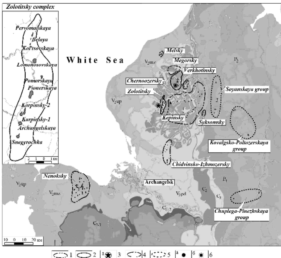
Fig. 1. The location of kimberlites, its convergent rocks and basaltic diatremes of Early-Hercynian complexes within Southern-Eastern White Sea region. 1-3 - Zimniberezhny Mega-Complex: 1 – Fe-Ti type (Kepinsky, Megorsy, Melsky, Chernoozersky Complexes); 2 – Mg-Al type (Zolotitsky, Verkhotinsky Complexes); 3 – Diamond deposits (1 – M.V. Lomonosov, 2 – V. Grib); 4 – Nenoksko-Chidvinsky Megacoplex (Nenoksky, Chidvinsko-Izhmoversky, Suksomsky Complexes); 5 – Soyana-Pinezhsky basaltic Complex pipes groups (Soyanskaya, Kovalgsko-Poltovskaya, Chuplega-Pinezhskaya); 6 – Diatremes: a – kimberlites, picrites, olivine melilitites, b – tholeiitic basalts.
