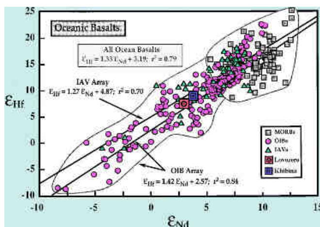
Fig. 10. \epsilon_{Nd} versus \epsilon_{Hf} isotopic composition of the Lovozero and Khibina ore minerals.
