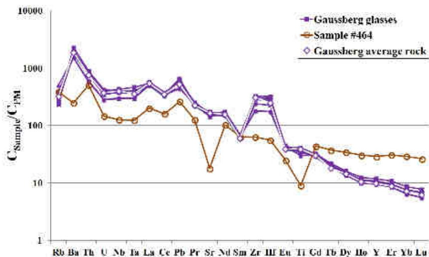
Fig.3. Lithophile element patterns of Gausberg glasses. PM after Sun & McDonough [1989].
