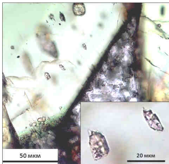
Figure 1. The primary melt inclusions in the clinopyroxene phenocrysts. Transmitted light image.
