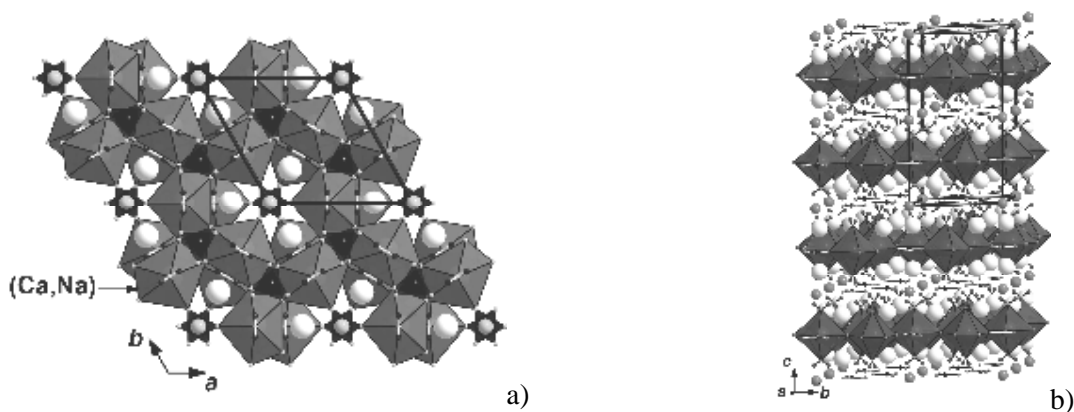
Figure 1. The crystal structure of alexkhomyakovite. CO_3 groups are black triangles, K cations are big light-grey spheres, Cl anions are medium-grey spheres, O anions are small grey circles and H atoms are small grey circles. The unit cell is outlined.
