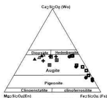
Fig. 3. Compositional variation of clinopyroxene of the ARC in the quadrilateral of pyroxenes. Fields and nomenclature are the one adopted by Deer et al. (1978). Symbol: as in figure 2.
