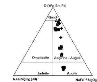
Fig. 2. Compositional variation of clinopyroxene of the ARC in the Jd-Q diagram. Fields and nomenclature after Morimoto (1988). Symbols: □-quartz syenite; ●-alkali syenite; nepheline syenite (◻-rim, +-core); alkali gabbro (▲-rim, ▲-core).
