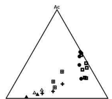
Fig. 4. Compositional variation of pyroxenes of the ARC in the Di-Ac-Hd diagram. Symbols as in figure 2.
