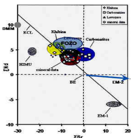
Fig. 9. \epsilon_{Nd} versus \epsilon_{Sr} isotopic composition of Lovozero and Khibina rocks.
