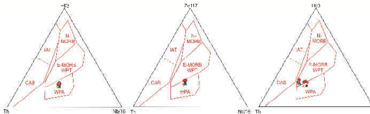
Fig 3. Th-Hf-Ta tectonomagmatic classification diagrams (Wood,1980) and plots of Şekeroba basanites.
