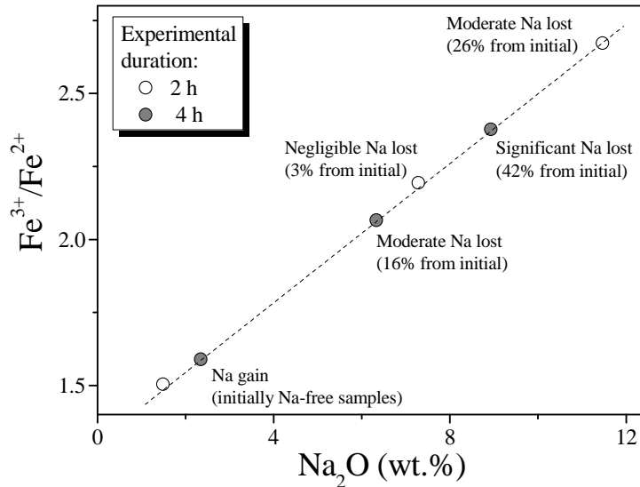
Fig. 1. Ferric/ferrous equilibrium in air at 1500°C in silicic melts (DAFS+Na series) suffering Na lost/Na gain.
