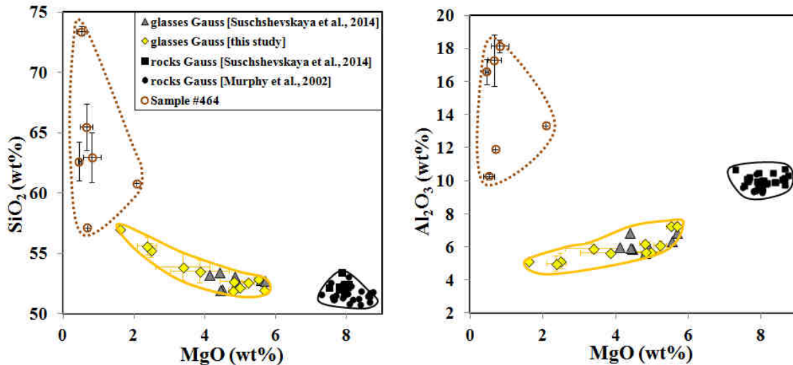
Fig.2. Major elements in quenched glasses and bulk rocks from Gaussberg volcano.
