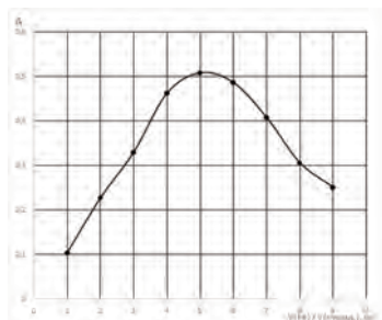
Fig. 2. Motorized series for the system Fe (II) – pyridoxine. C(BPS) = 5 \cdot 10^{-5} mol / l, pH = 7.0, \lambda = 440 nm, l = 0.5 cm, PE - 5400 (in a ditch of comparison With(Bureau) = 1 \cdot 10^{-5} mol / l)
