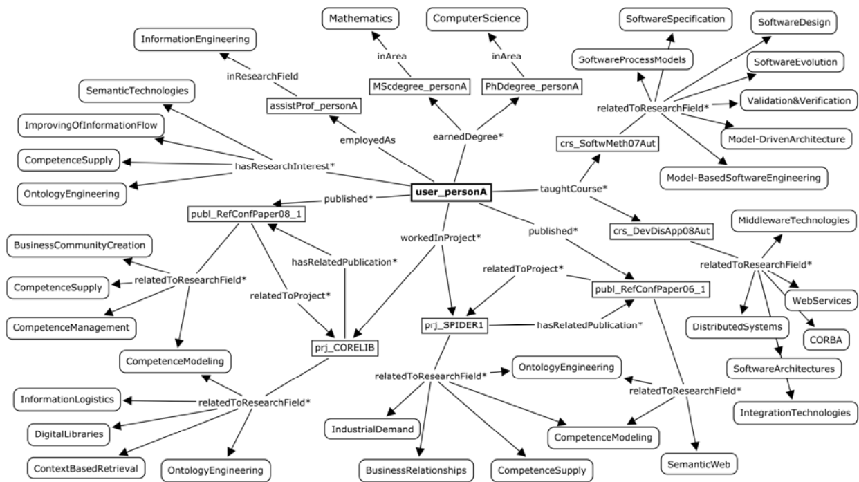
Figure 2. Example of a user profile for person A
