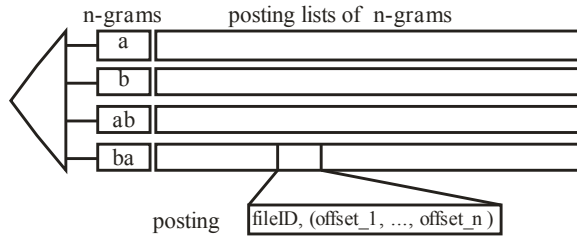
Figure 2: n-gram index.
