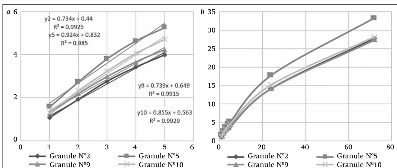
Fig.2. The granule's hygroscopicity of compositions N° 2, 5, 9 and 10 (relative humidity of air of 98%): a – 5 hours; b – 72 hours. X-axis : time, hours; Y-axis : moisture absorption, %.)
