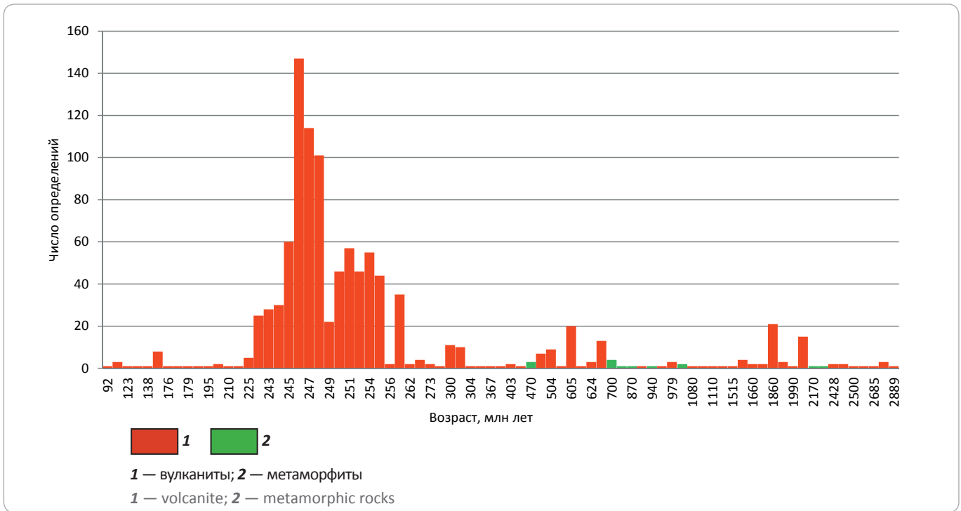
Fig. 4. Dating distribution for zircon of different genesis from volcanite (Zone I) and metamorphic rocks in the southern zone (Zone II)
