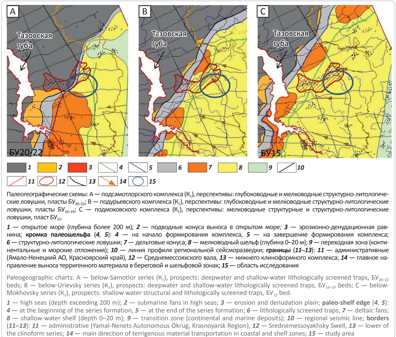
Fig. 2. Paleogeographic charts of clinoform series within the Srednemesoyakhsky Swell (prepared basing on R&D data obtained under the direction of Igoshkin V.P., 2007)
