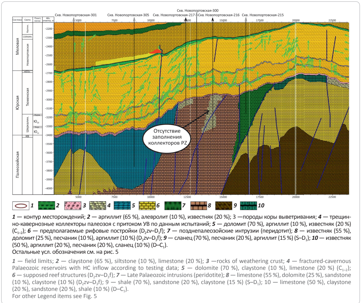
Fig. 7. 2D geological cross-section along the seismic slalom line in the Novoportovskiy area showing migration directions and HC accumulation zones
