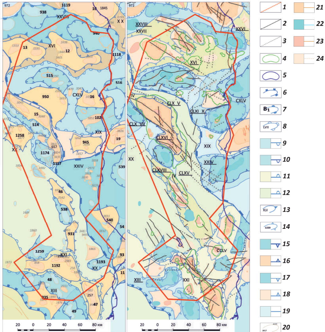
Fig. 5. Tectonic scheme of the eastern Yamal sedimentary cover: after V.S. Bochkarev (1990) (A) and created on the results of researches completed by the authors (B)
